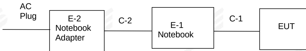
Conducted Emission Test
