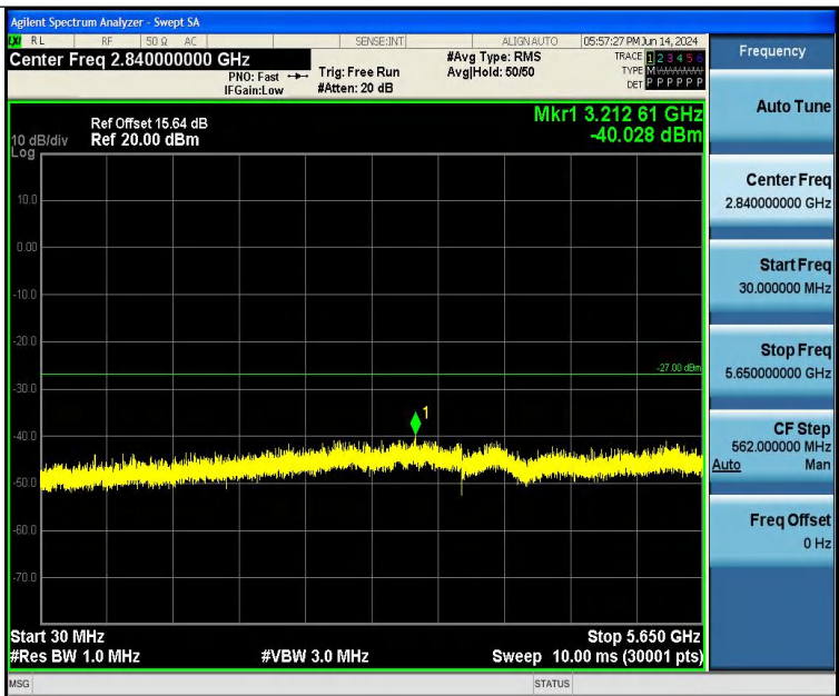
11N40SISO-Ant1-5795-30~5650-PASS
