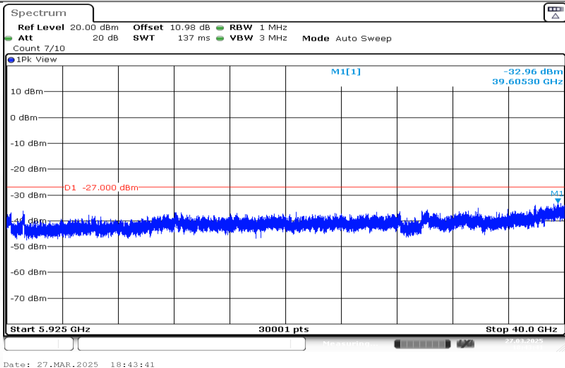
11AX40-Ant1-5755-5925~40000-PASS
