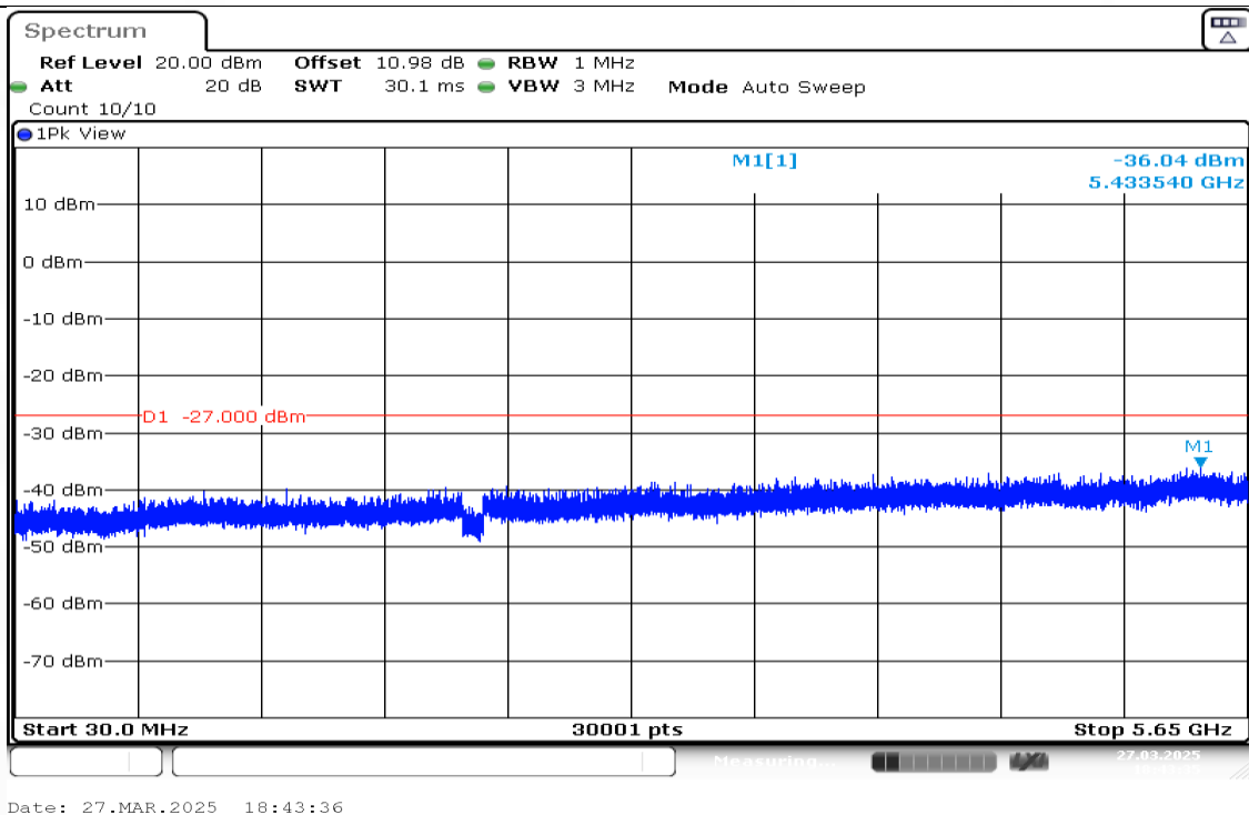
11AX40-Ant1-5755-30~5650-PASS
