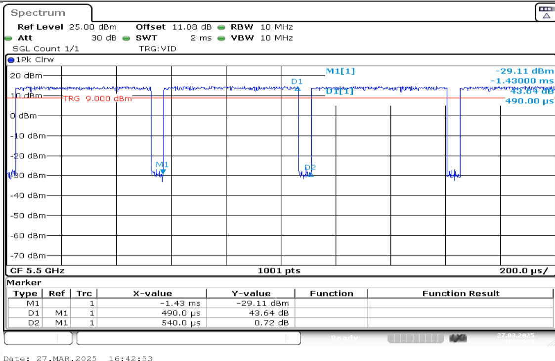
NTNV-11AX20MIMO-Ant2-5500
