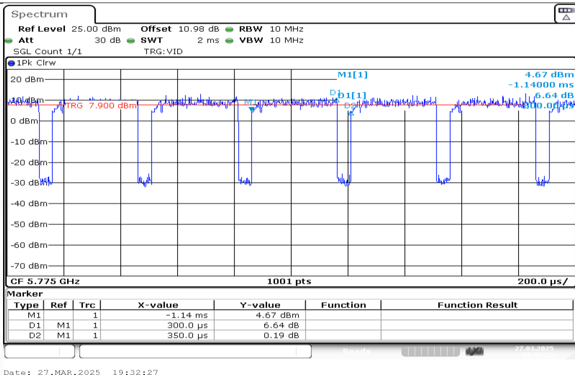
NTNV-11AX80MIMO-Ant1-5775
