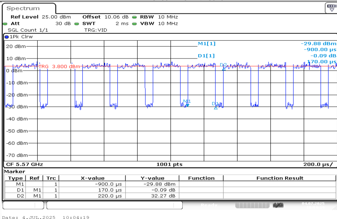
NTNV-11AC160MIMO-Ant2-5570
