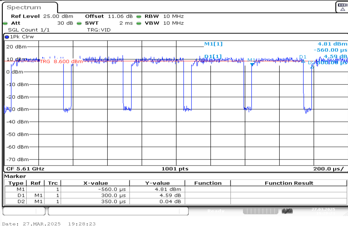
NTNV-11AX80MIMO-Ant2-5610
