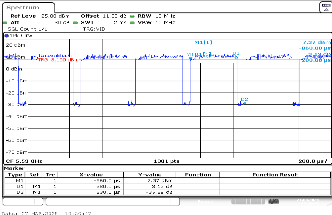
NTNV-11AX80MIMO-Ant2-5530
