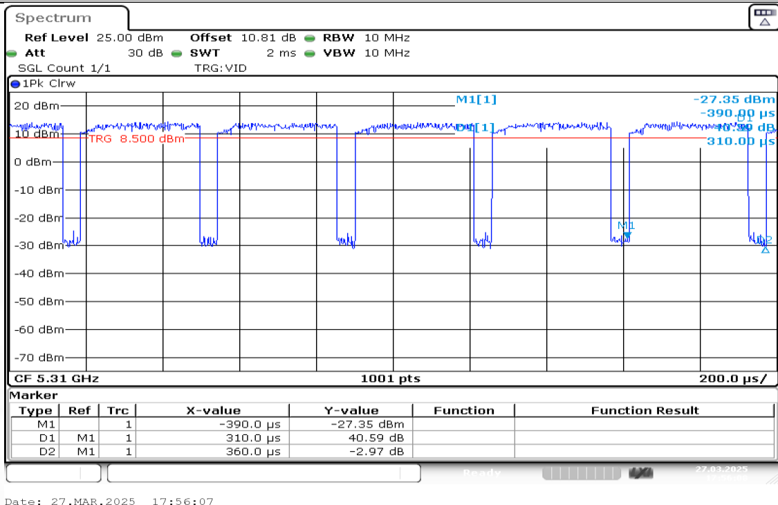
NTNV-11AX40MIMO-Ant2-5310
