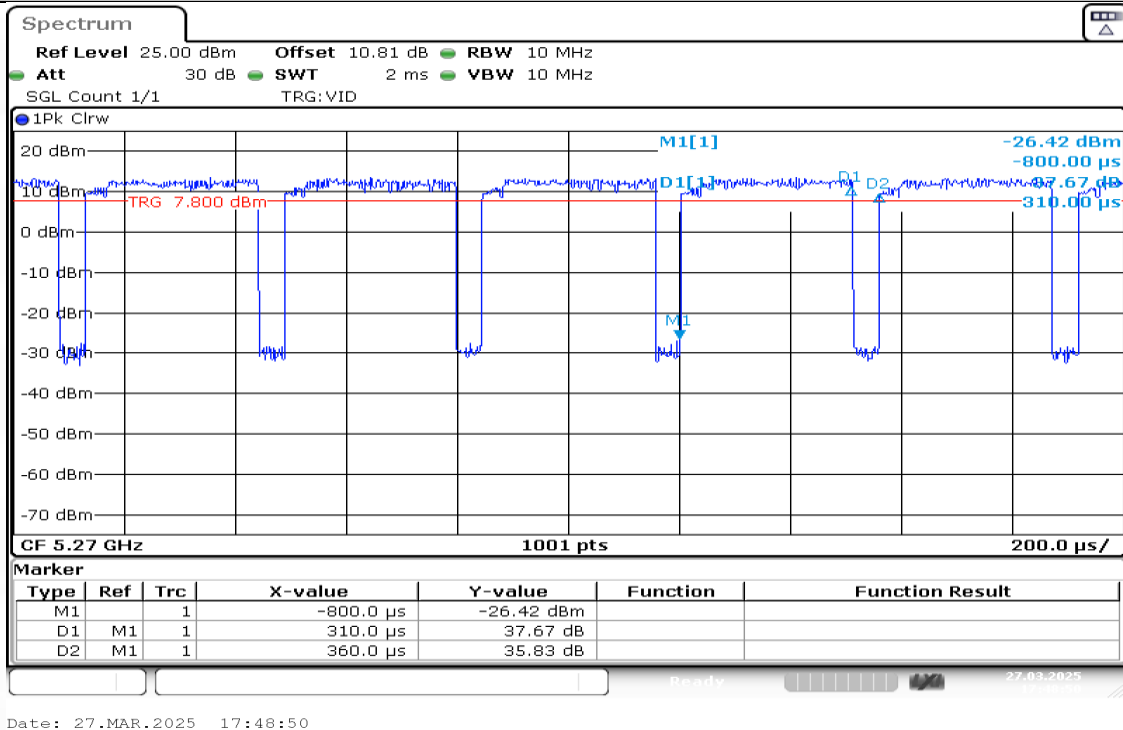
NTNV-11AX40MIMO-Ant2-5270
