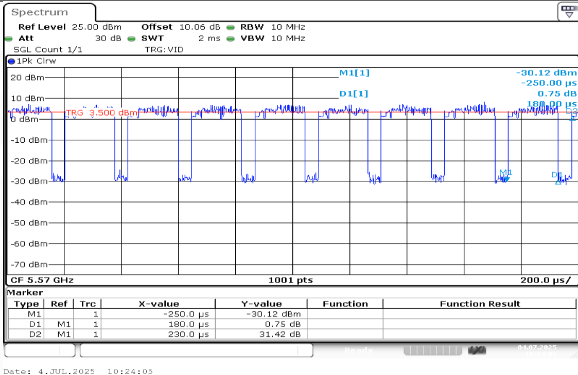
NTNV-11AX160MIMO-Ant2-5570
