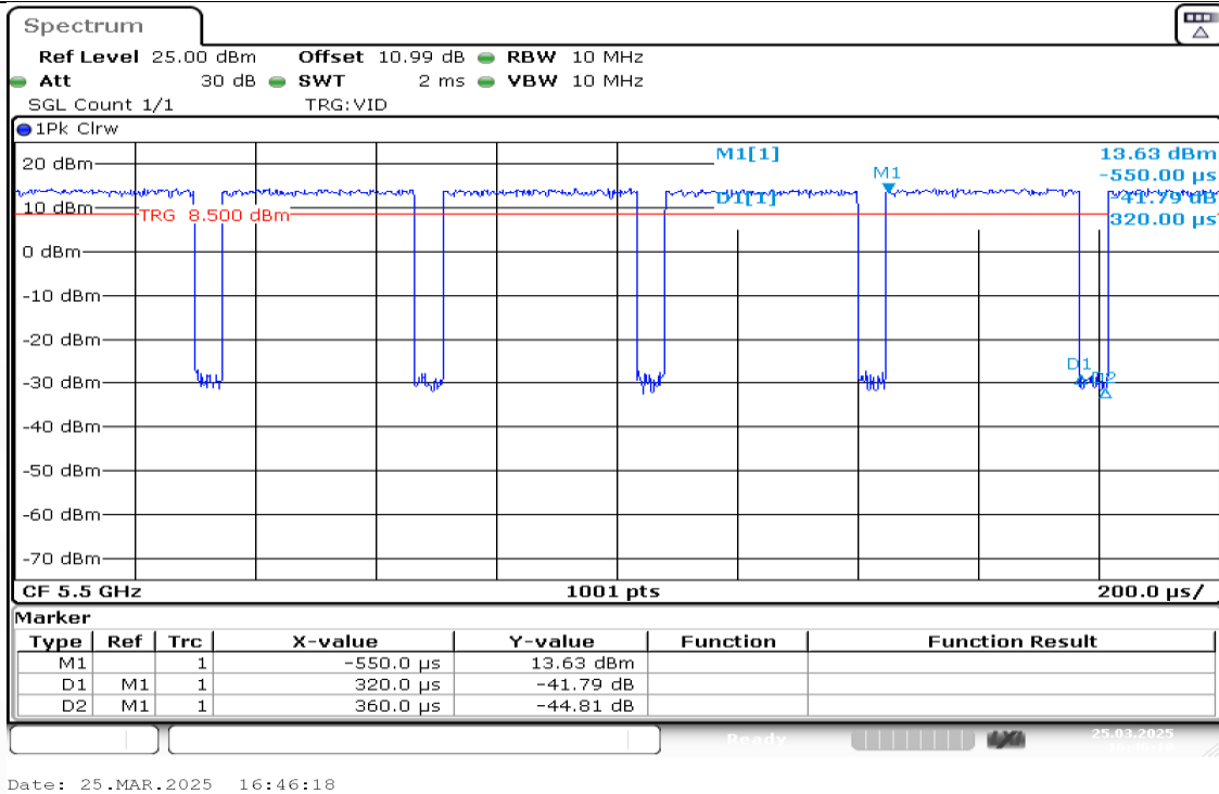
NTNV-11AC20MIMO-Ant1-5500
