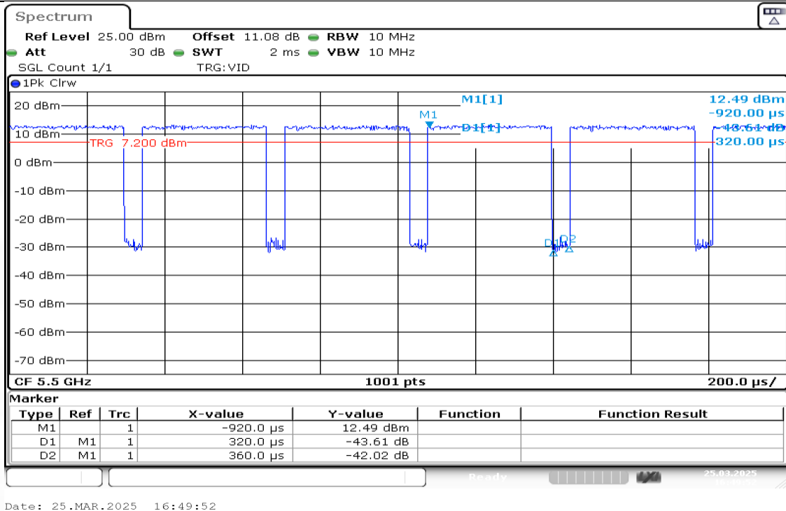
NTNV-11AC20MIMO-Ant2-5500
