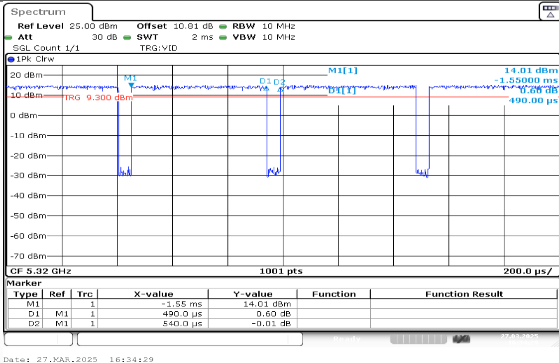
NTNV-11AX20MIMO-Ant2-5320
