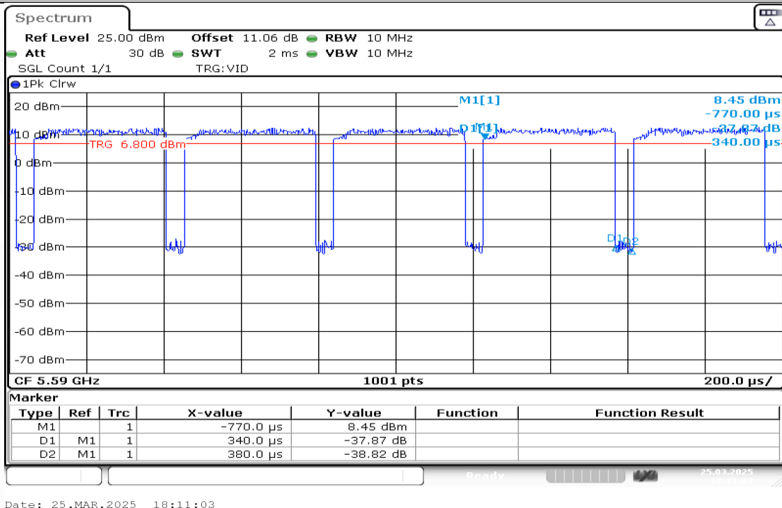
NTNV-11AC40MIMO-Ant2-5590
