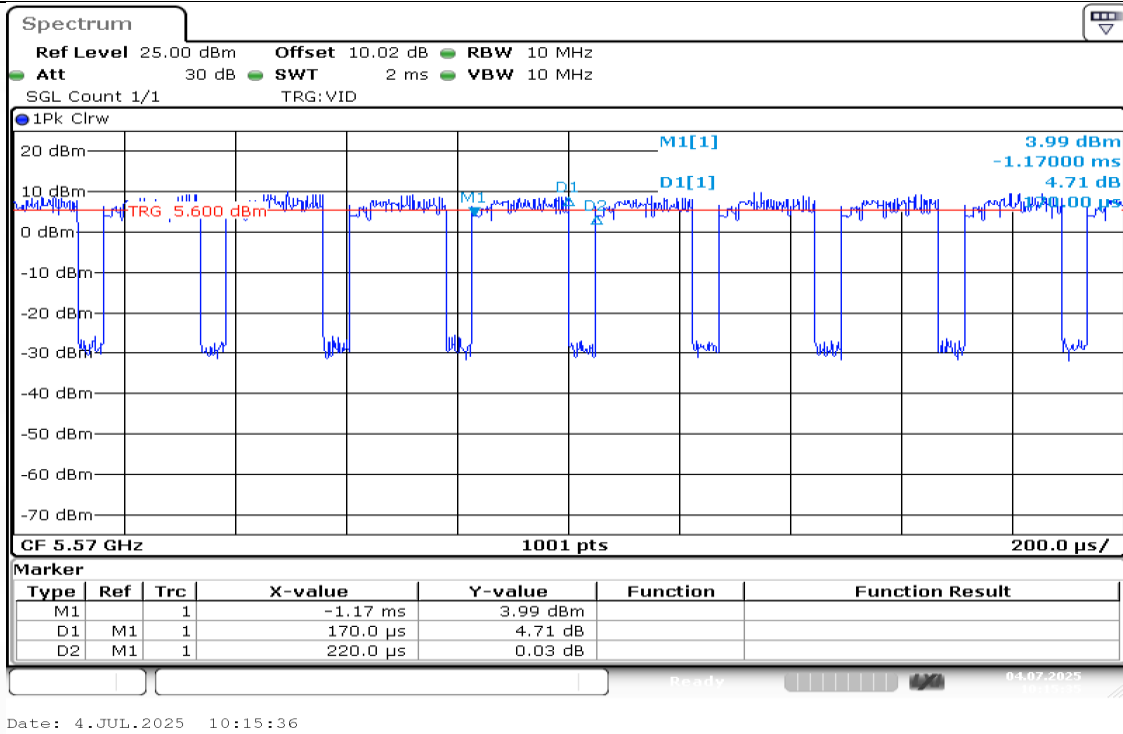
NTNV-11AX160MIMO-Ant1-5570
