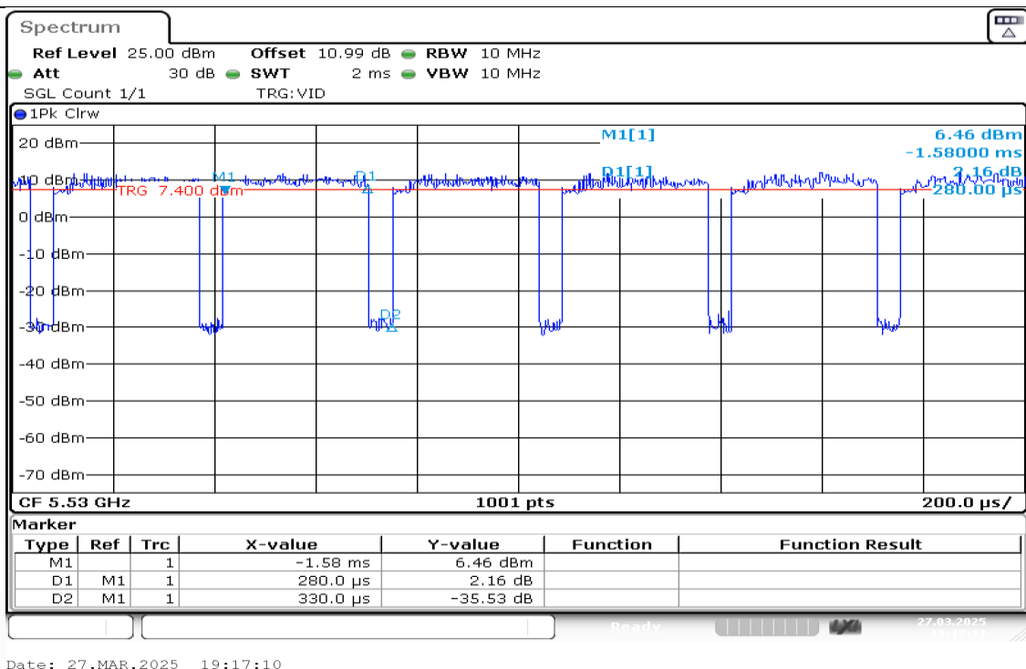
NTNV-11AX80MIMO-Ant1-5530
