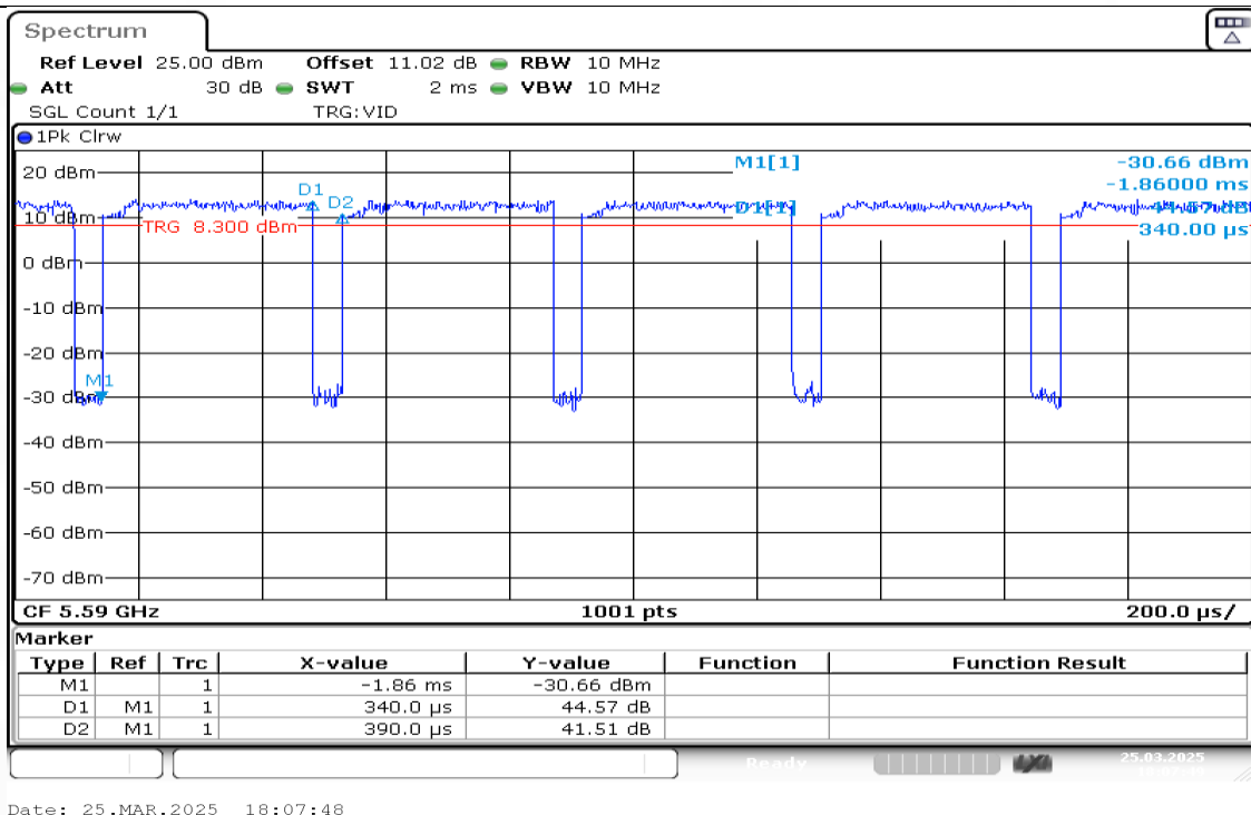
NTNV-11AC40MIMO-Ant1-5590
