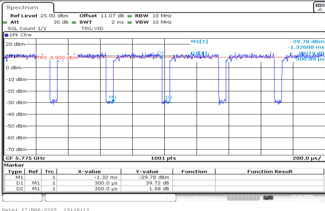
NTNV-11AX80MIMO-Ant2-5775
