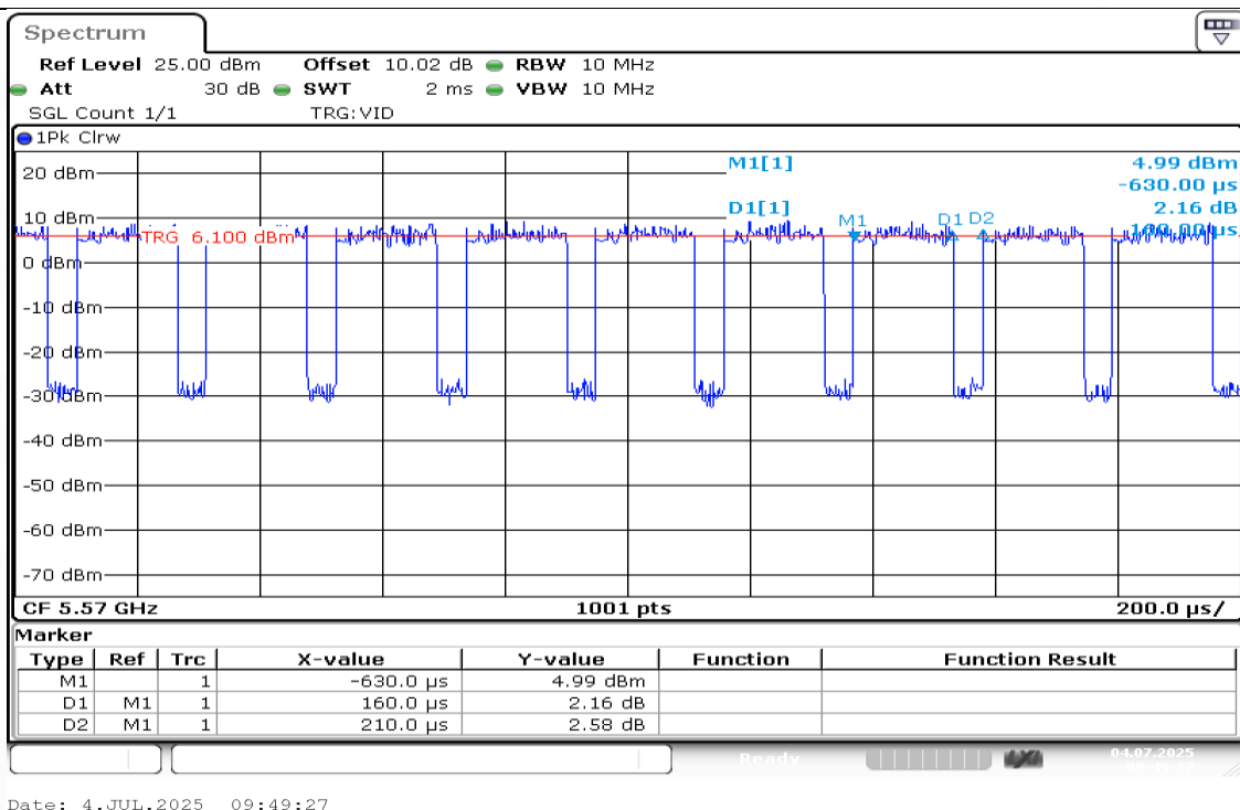
NTNV-11AC160MIMO-Ant1-5570
