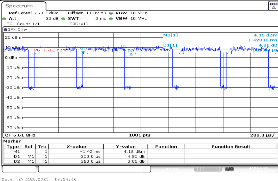
NTNV-11AX80MIMO-Ant1-5610
