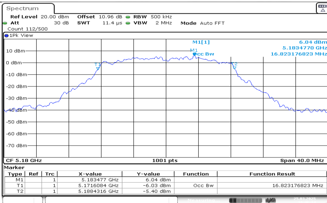
11A-Ant1-5180
