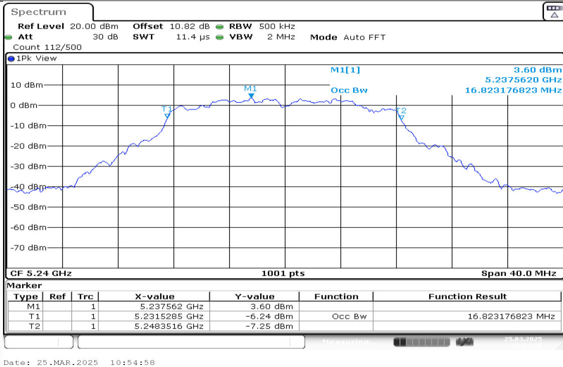
11A-Ant1-5240
