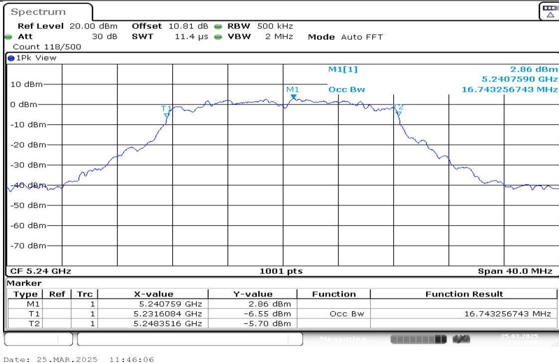
11A-Ant2-5240
