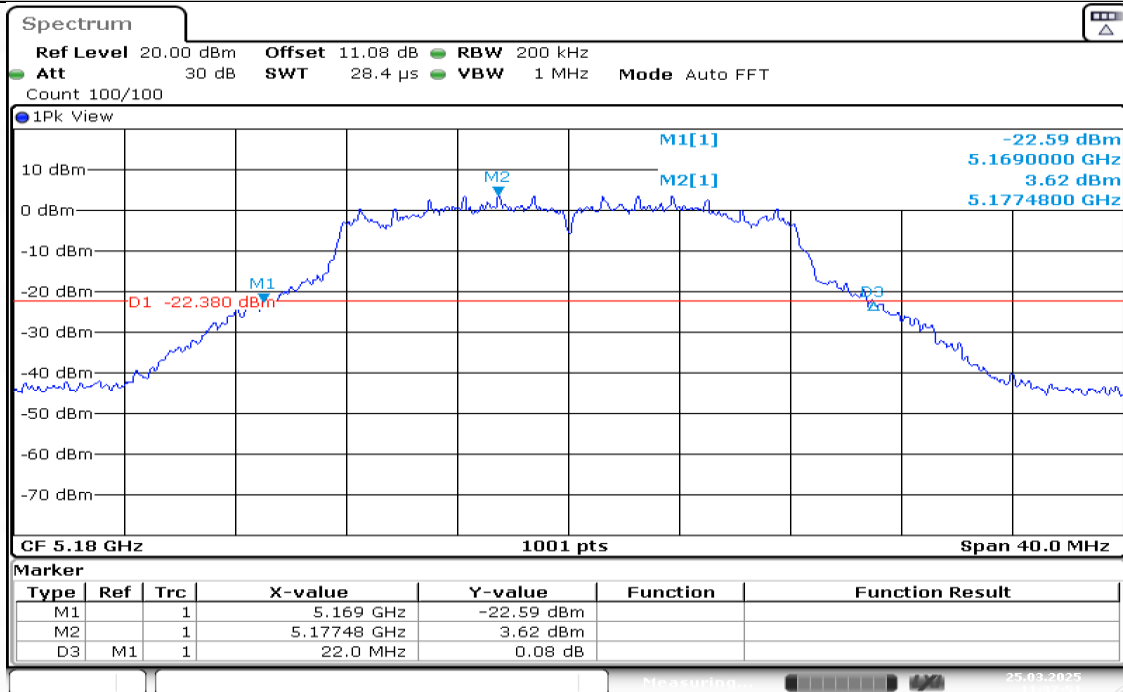
11A-Ant1-5180
