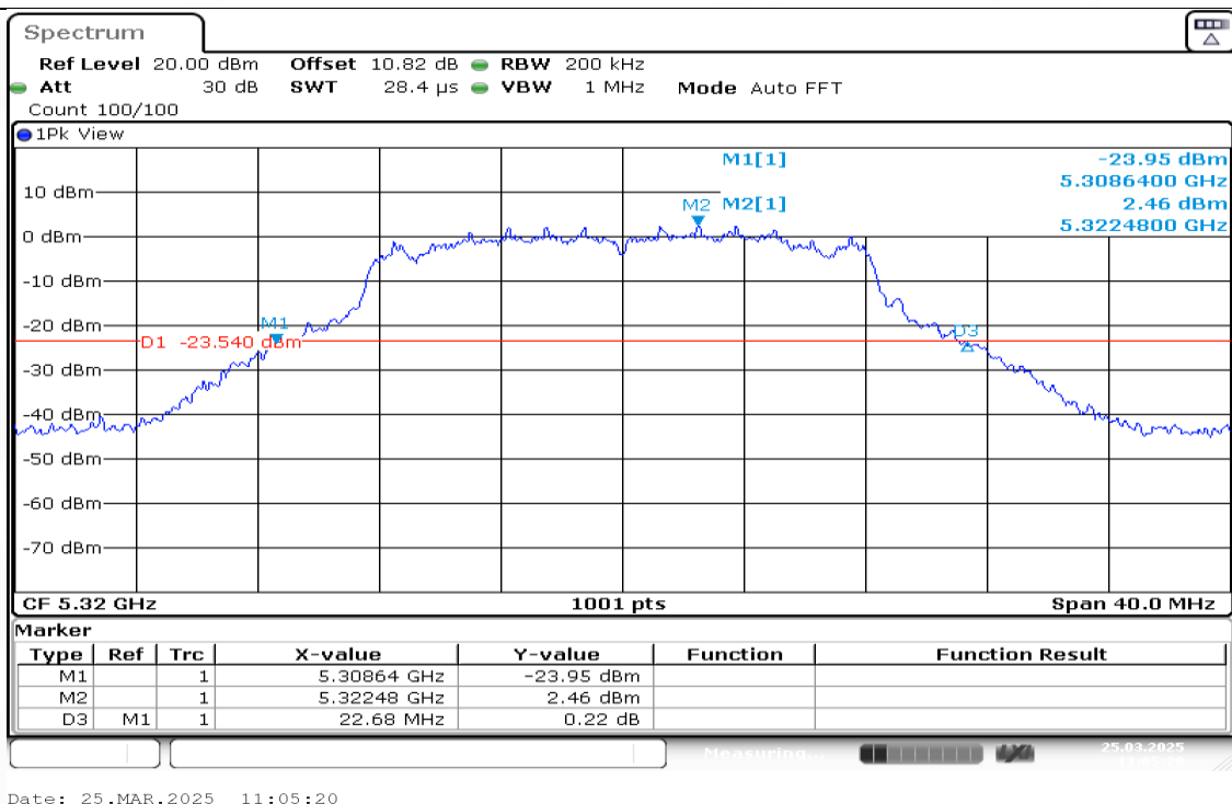
11A-Ant1-5320
