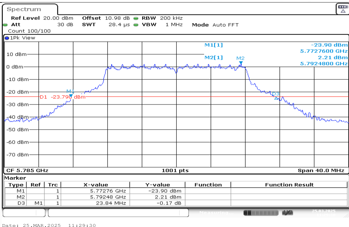
11A-Ant1-5785
