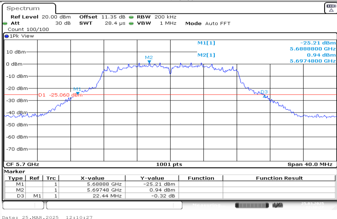
11A-Ant2-5700
