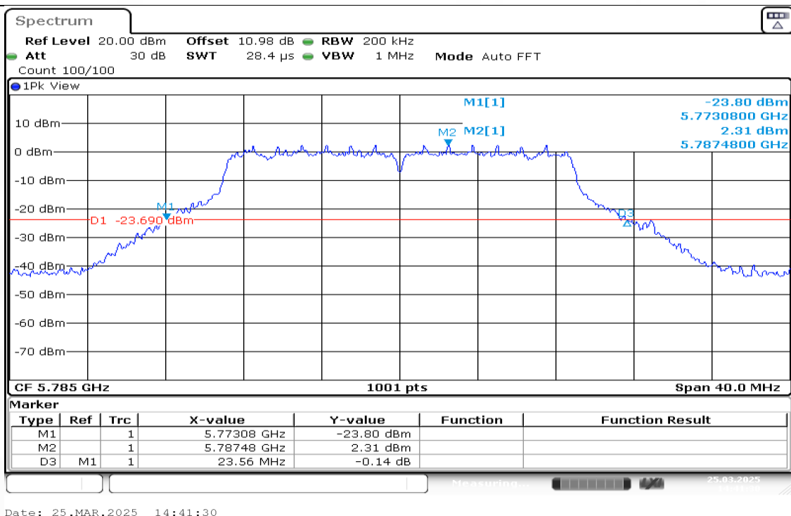
11N20MIMO-Ant1-5785
