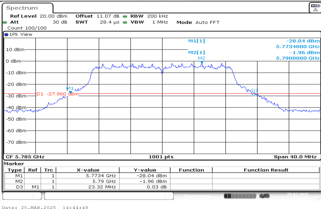
11N20MIMO-Ant2-5785
