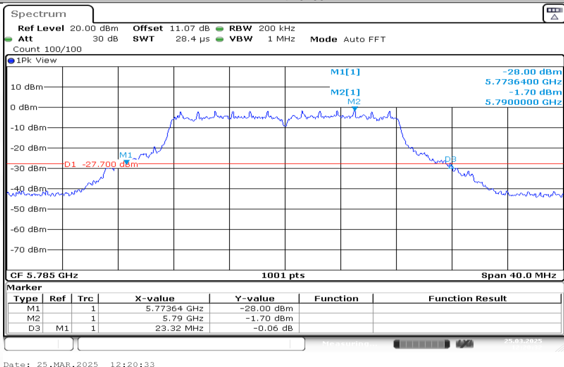
11A-Ant2-5785
