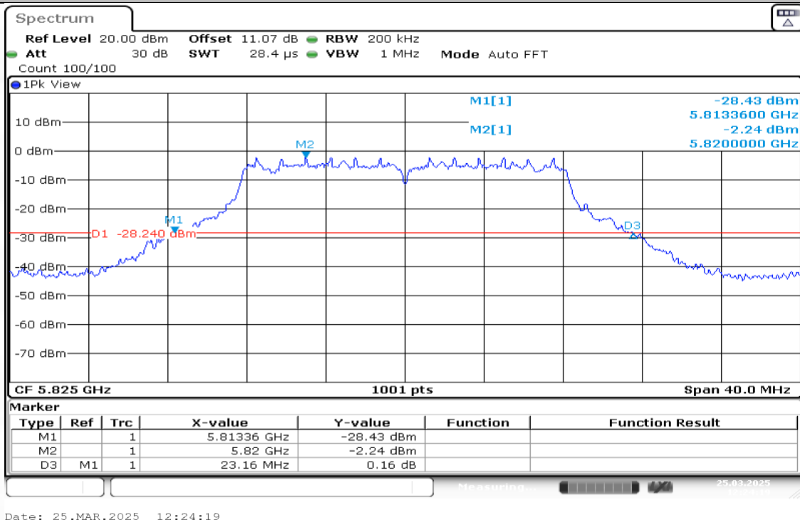
11A-Ant2-5825
