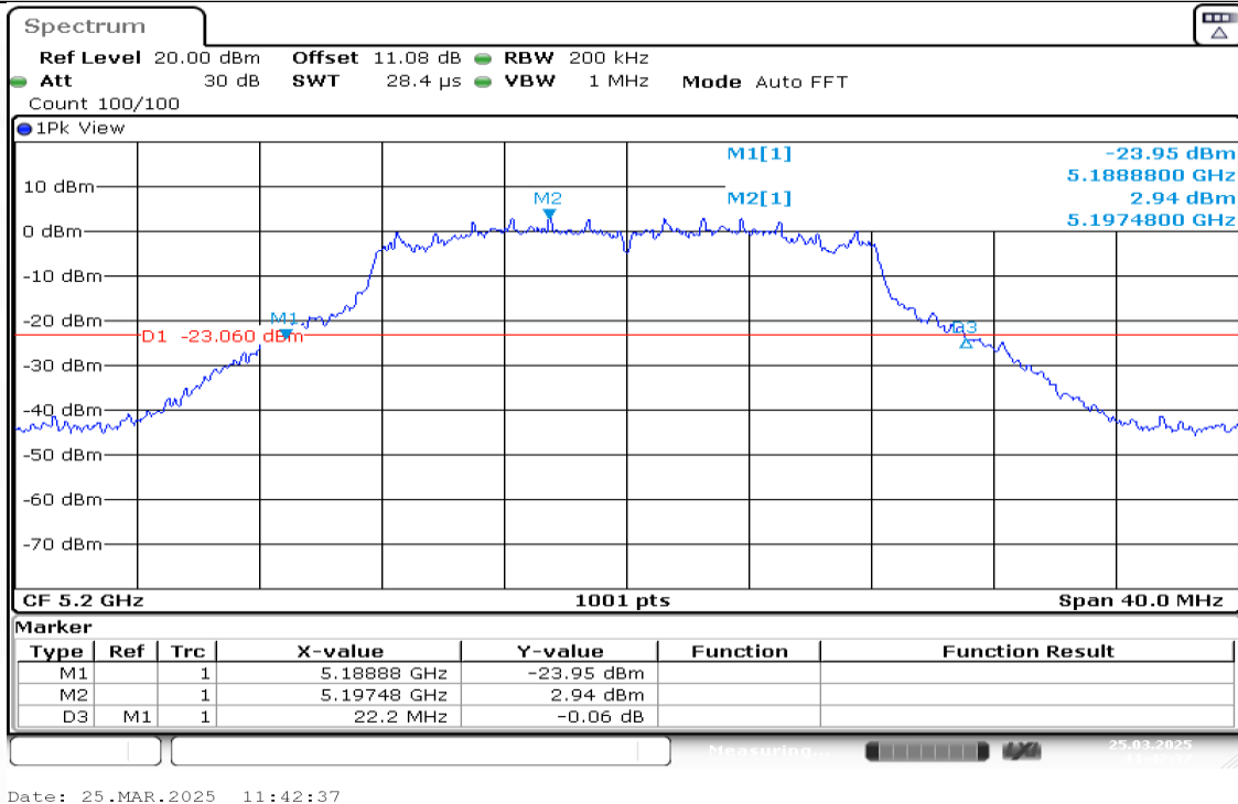
11A-Ant2-5200
