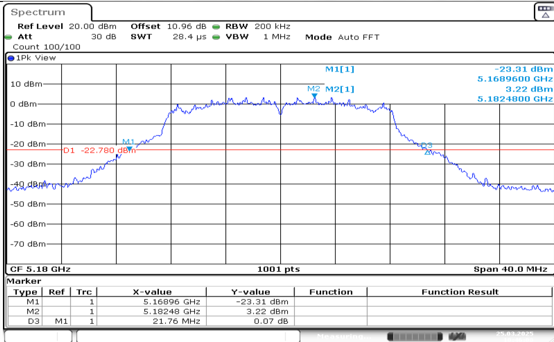
11A-Ant1-5180
