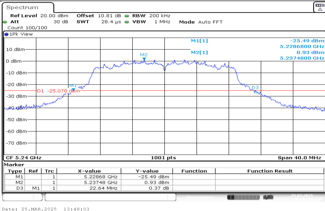
11N20MIMO-Ant2-5240
