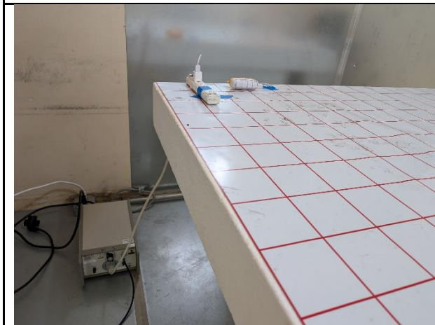
AC Power Line Conducted Emission-Front
