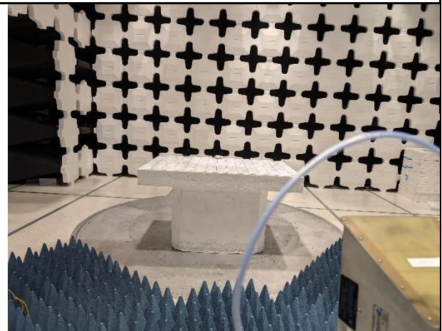
Radiated Emission-Above 1GHz-Back
