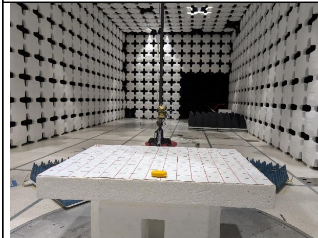
Radiated Emission-Above 1GHz-Front
