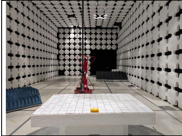
Radiated Emission-Below 1GHz-Front
