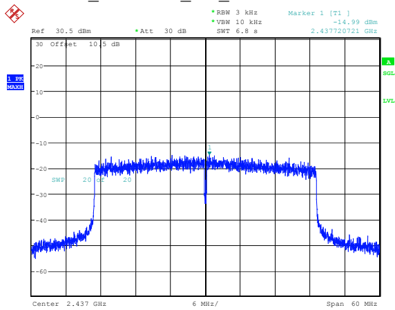
802.11ax40_2437MHz_RU_Full -14.99dBm/3kHz
