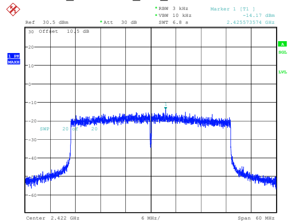
802.11ax40_2422MHz_RU_Full -14.17dBm/3kHz
