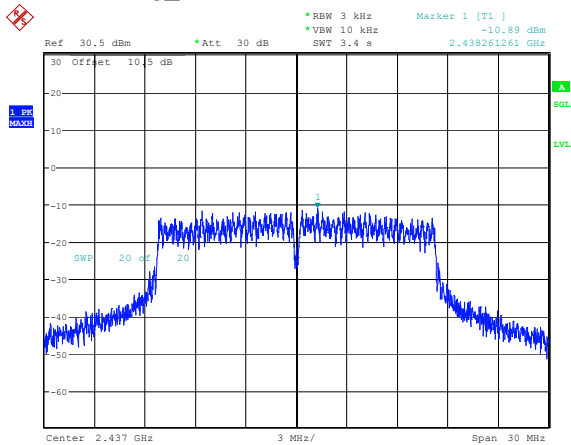
802.11g_2437MHz -10.89dBm/3kHz
