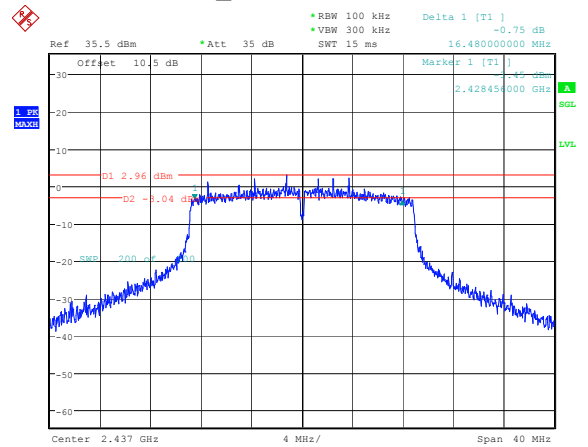
802.11n20_2437MHz 16.480MHz
