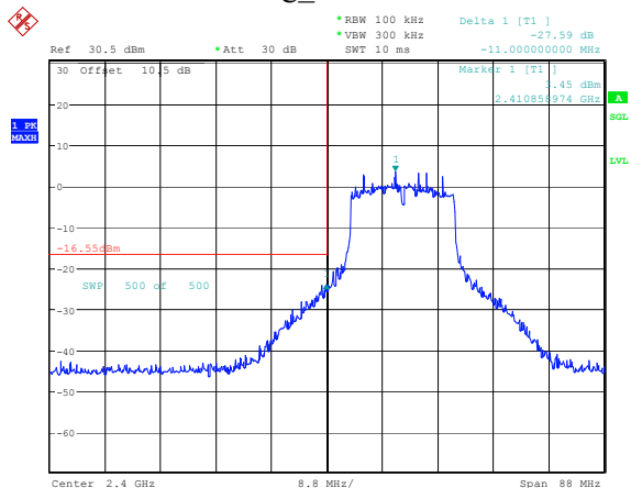
802.11g 2412MHz
