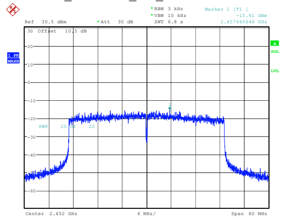
802.11ax40_2452MHz_RU_Full -15.41dBm/3kHz
