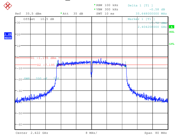
802.11n40_2422MHz 35.648MHz
