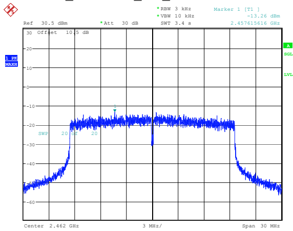
802.11ax20_2462MHz_RU_Full -13.26dBm/3kHz
