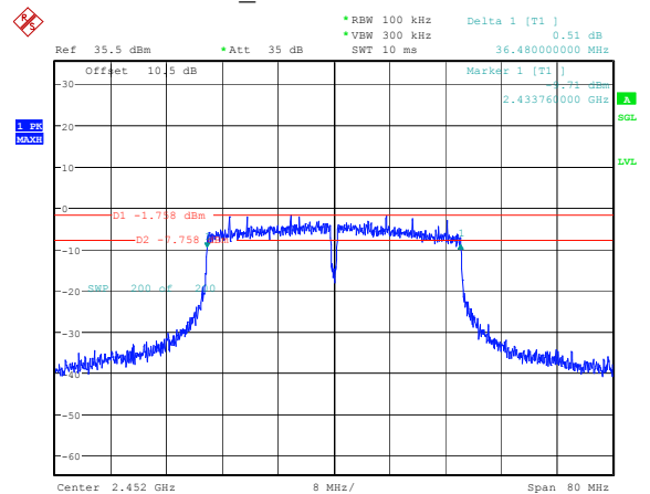
802.11n40_2452MHz 36.480MHz
