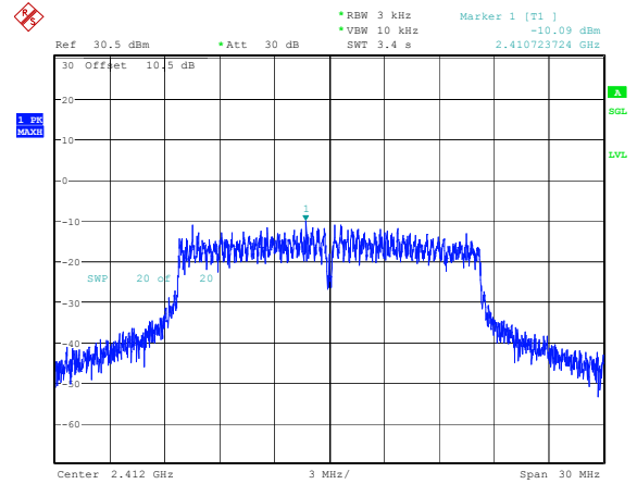
802.11g_2412MHz -10.09dBm/3kHz
