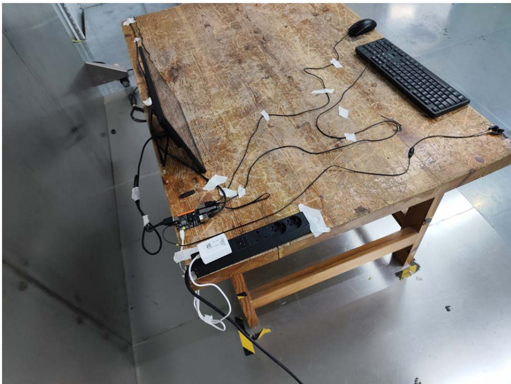
Conducted Emissions Side View RDK X5 4G
