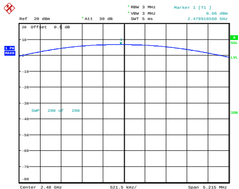
GFSK_High 6.66dBm
