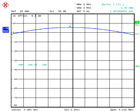
GFSK_Low 5.30dBm
