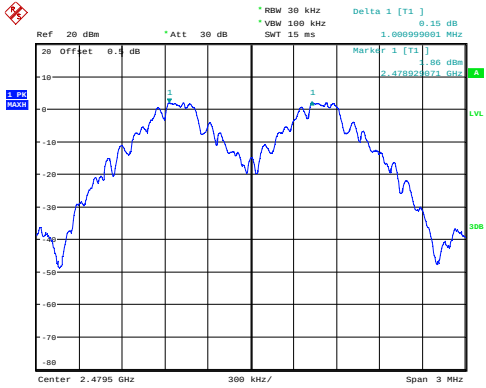
GFSK_High 1.001MHz
