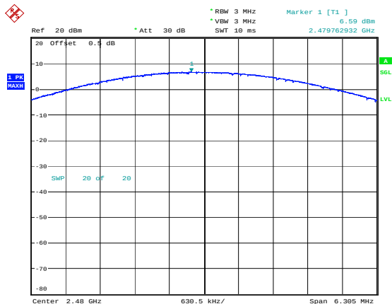
\pi/4 -DQPSK_High 6.59dBm
