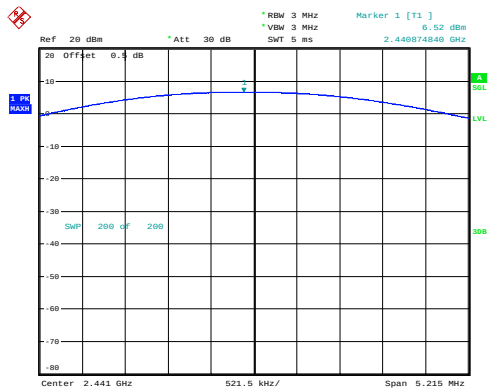
GFSK_Middle 6.52dBm
