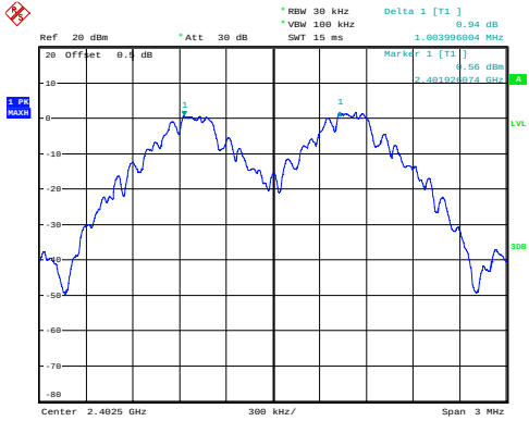
GFSK_Low 1.004MHz
