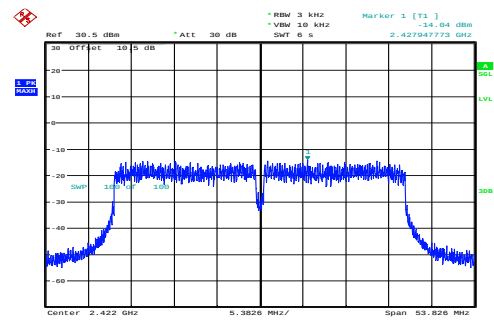
n40_2422MHz_Chain 0 -14.04dBm/3kHz
