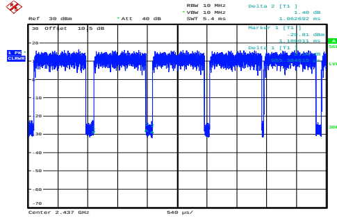
n40_2437MHz_Chain 0 0.955ms,1.063ms
