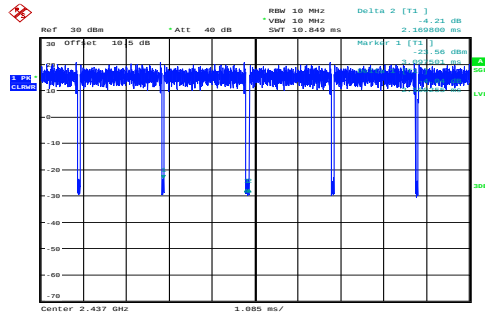
g_2437MHz_Chain 0 2.100ms,2.170ms
