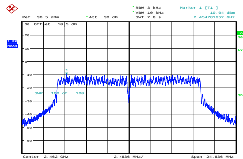
g_2462MHz_Chain 0 -10.04dBm/3kHz
