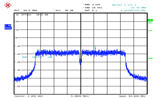
n40_2452MHz_Chain 0 -13.73dBm/3kHz
