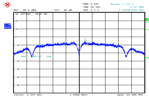
b_2437MHz_Chain 0 -5.87dBm/3kHz
