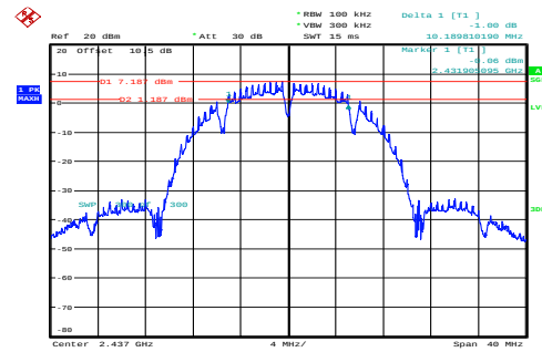
b_2437MHz_Chain 0 10.190MHz
