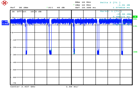
n20_2437MHz_Chain 0 1.946ms,1.980ms
