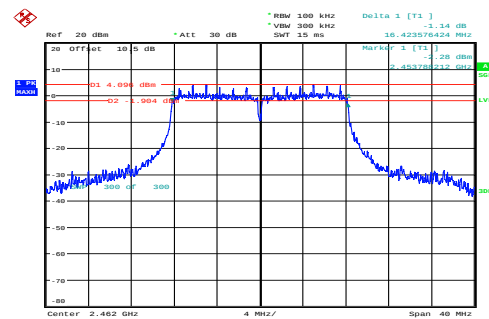
g_2462MHz_Chain 0 16.424MHz
