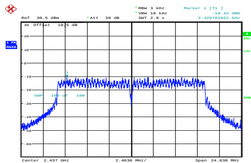
g_2437MHz_Chain 0 -10.42dBm/3kHz
