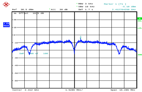
b_2412MHz_Chain 0 -5.10dBm/3kHz
