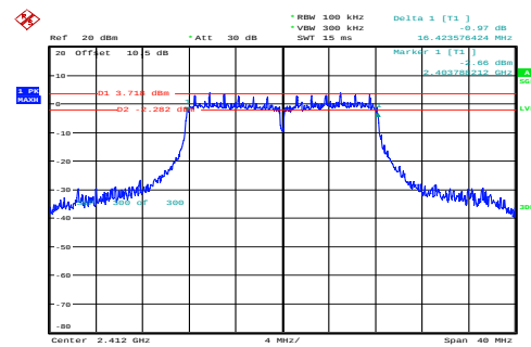
g_2412MHz_Chain 0 16.424MHz
