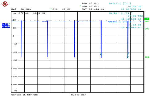
b_2437MHz_Chain 0 12.599ms,12.637ms
