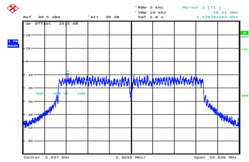
n20_2437MHz_Chain 0 -10.41dBm/3kHz
