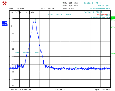
GFSK_High 59.35dB
