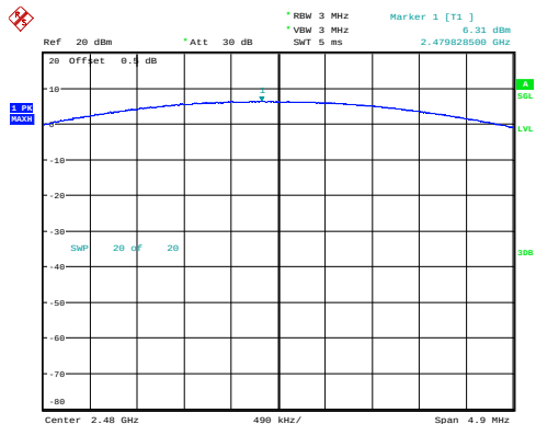
GFSK_High 6.31dBm
