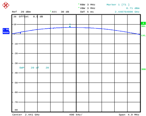
GFSK_Middle 6.71dBm
