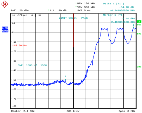
GFSK_Hopping_Lower 54.10dB
