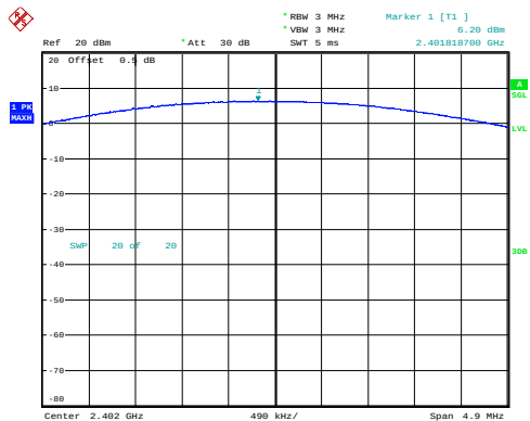
GFSK_Low 6.20dBm
