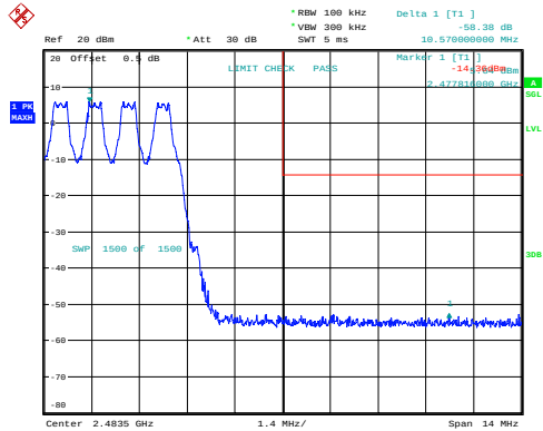
GFSK_Hopping_Upper 58.38dB
