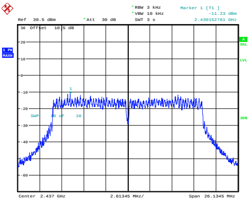
n20_2437MHz_Chain 0 -11.23dBm/3kHz
