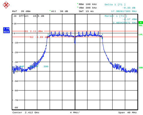
n20_2412MHz_Chain 0 17.383MHz
