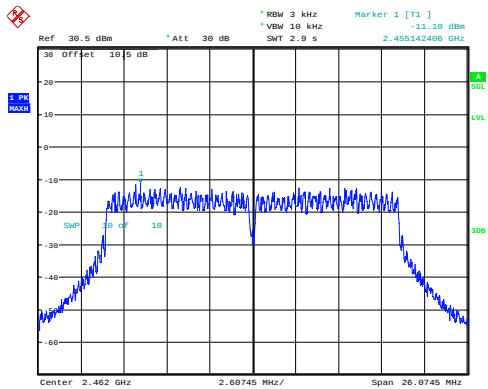
n20_2462MHz_Chain 0 -11.10dBm/3kHz
