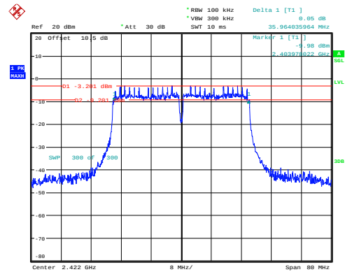
n40_2422MHz_Chain 0 35.964MHz
