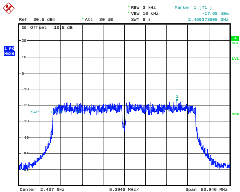
n40_2437MHz_Chain 0 -17.68dBm/3kHz
