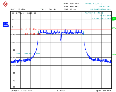
n40_2452MHz_Chain 0 35.964MHz
