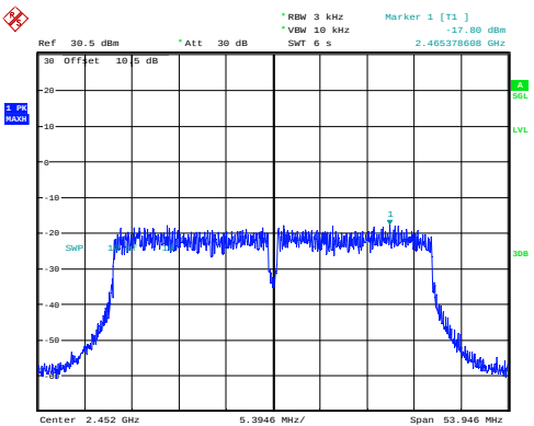
n40_2452MHz_Chain 0 -17.80dBm/3kHz
