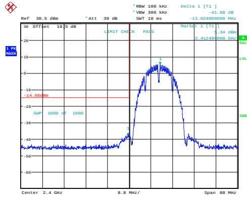
b_2412MHz_Chain 0 41.68dB
