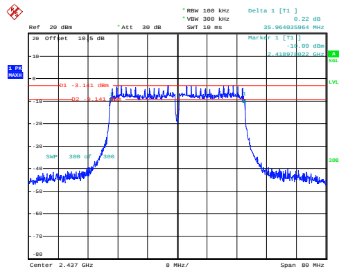
n40_2437MHz_Chain 0 35.964MHz
