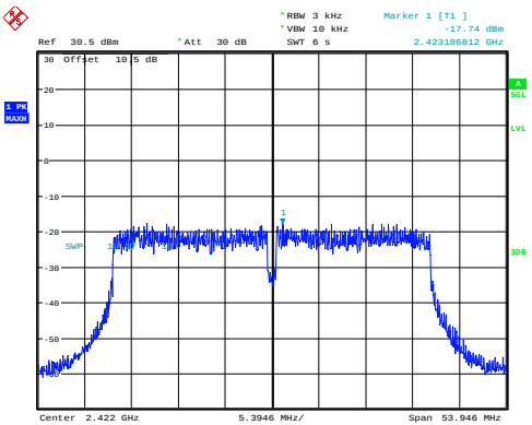
n40_2422MHz_Chain 0 -17.74dBm/3kHz
