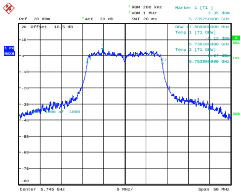
n20_5745MHz_Chain 0 17.800MHz
