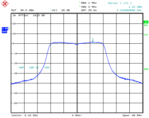
a_5240MHz_Chain 0 1.32dBm/MHz
