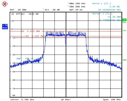
n40_5795MHz_Chain 0 36.164MHz
