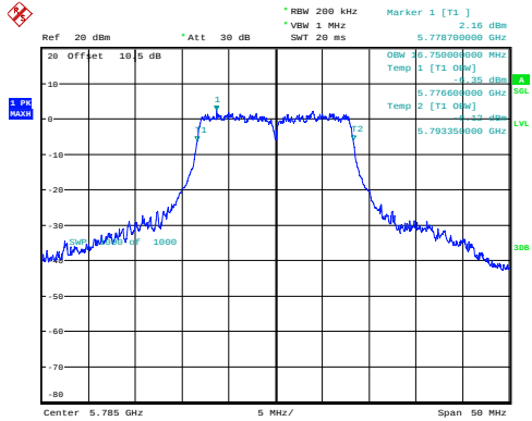
a_5785MHz_Chain 0 16.750MHz
