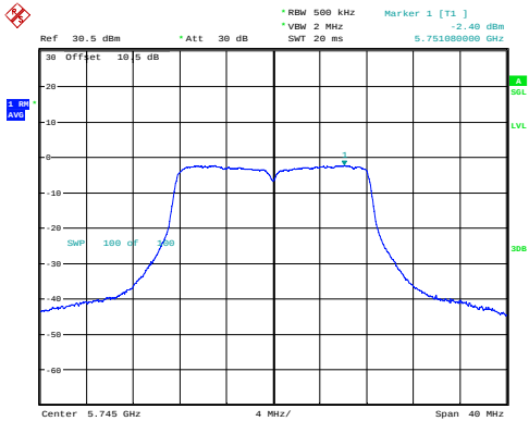
a_5745MHz_Chain 0 -2.40dBm/MHz
