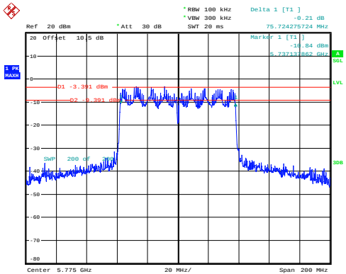
ac80_5775MHz_Chain 0 75.724MHz
