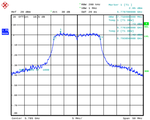
n20_5785MHz_Chain 0 17.750MHz
