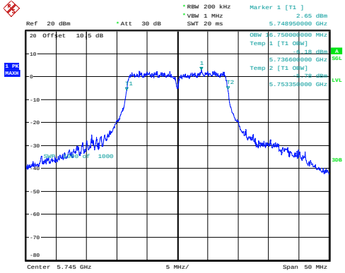
a_5745MHz_Chain 0 16.750MHz
