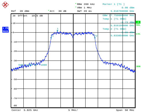
n20_5825MHz_Chain 0 17.750MHz
