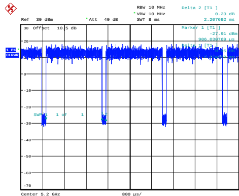
a_5200MHz_Chain 0 2.074ms,2.208ms
