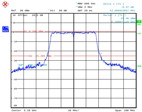
n40_5190MHz_Chain 0 43.057MHz
