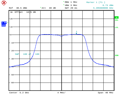
n20_5200MHz_Chain 0 0.73dBm/MHz
