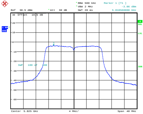
n20_5825MHz_Chain 0 -3.86dBm/MHz
