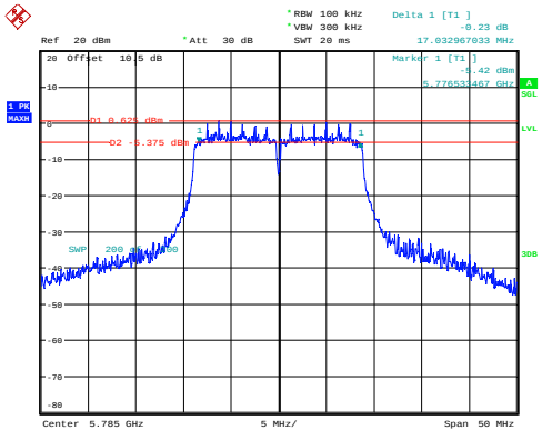
n20_5785MHz_Chain 0 17.033MHz
