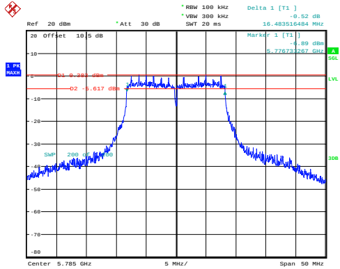
a_5785MHz_Chain 0 16.484MHz
