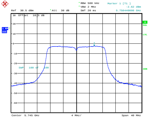
n20_5745MHz_Chain 0 -2.62dBm/MHz
