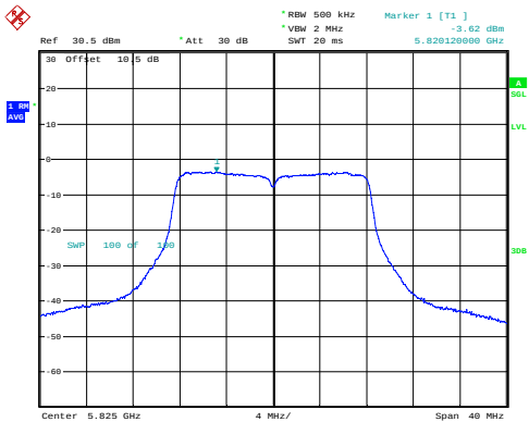
a_5825MHz_Chain 0 -3.62dBm/MHz
