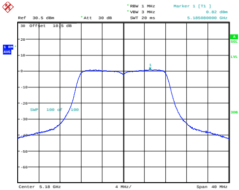
a_5180MHz_Chain 0 0.82dBm/MHz
