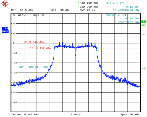
a_5745MHz_Chain 0 16.484MHz
