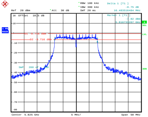
a_5825MHz_Chain 0 16.484MHz
