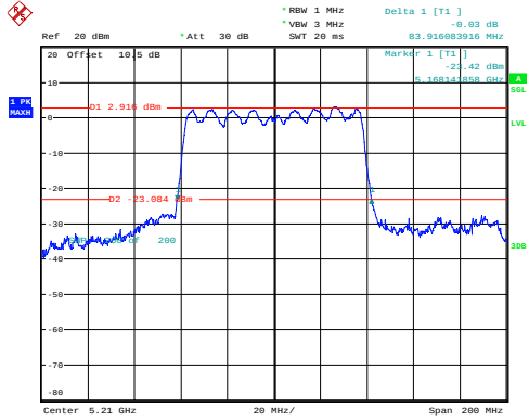
ac80_5210MHz_Chain 0 83.916MHz
