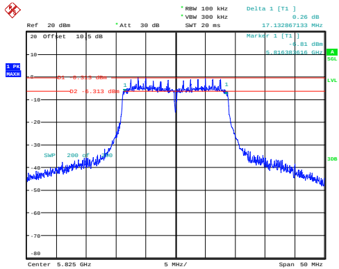
n20_5825MHz_Chain 0 17.133MHz
