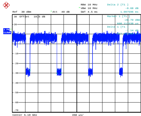
n40_5190MHz_Chain 0 0.958ms,1.098ms
