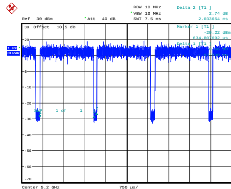
n20_5200MHz_Chain 0 1.938ms,2.034ms
