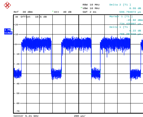
ac80_5210MHz_Chain 0 0.465ms,0.597ms
