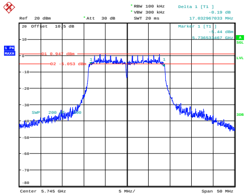
n20_5745MHz_Chain 0 17.033MHz
