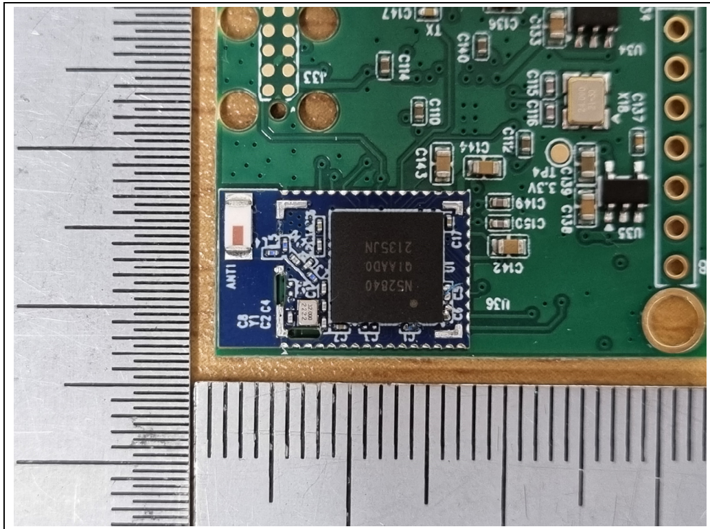
<BLE Module and Antenna>
