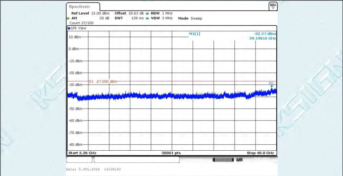
11AC20SISO_Ant1_5220_5360~40000
