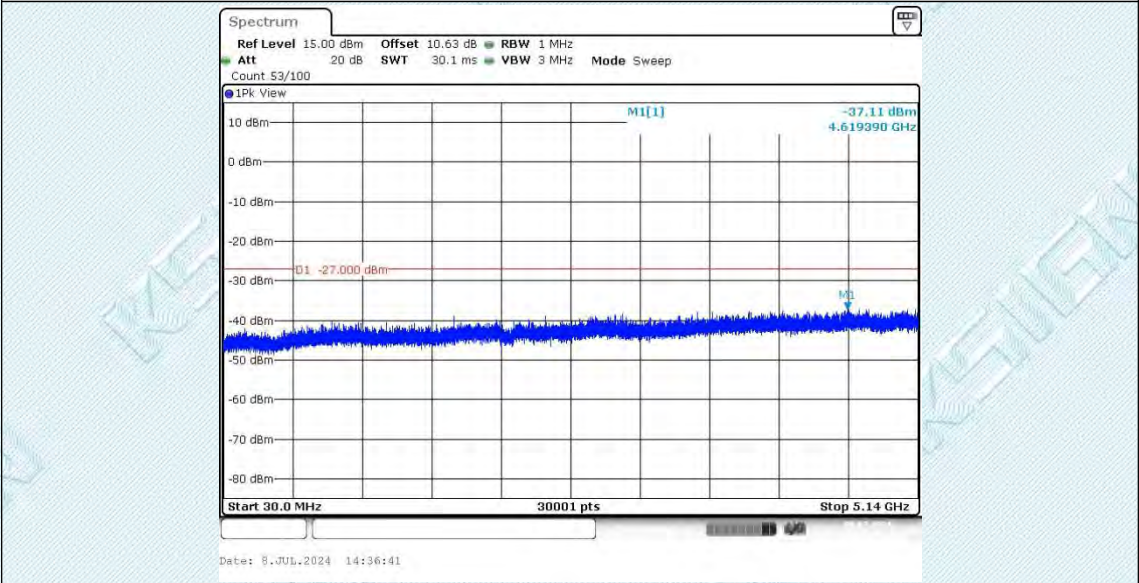
11AC40SISO_Ant1_5230_30~5140
