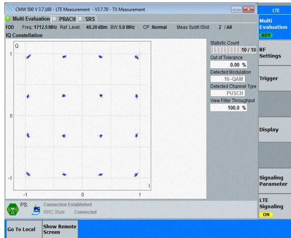
Band66-5MHz-16QAM-132322-25RB#0
