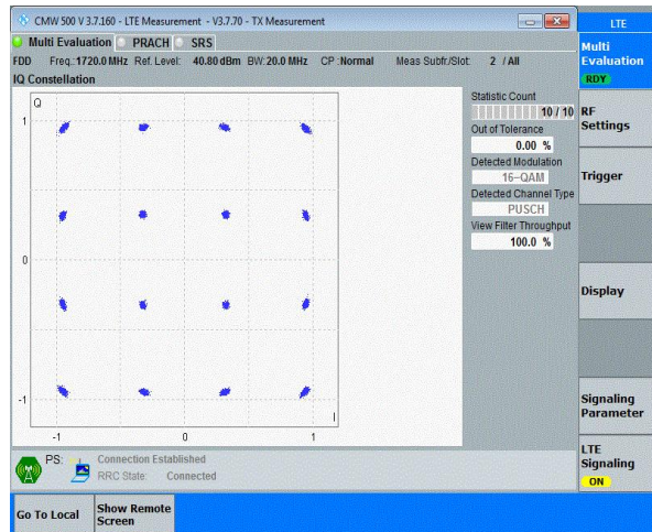
Band66-20MHz-16QAM-132322-100RB#0
