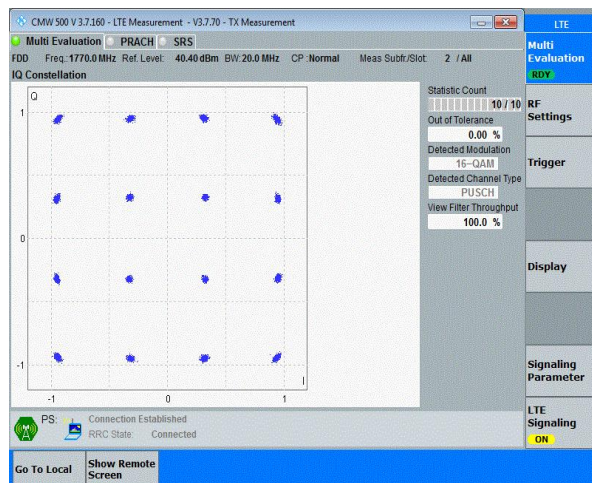
Band66-20MHz-16QAM-132572-100RB#0
