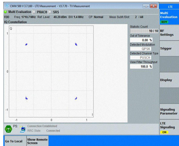
Band4-1.4MHz-QPSK-20175-6RB#0
