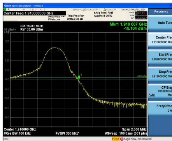
Band2-5MHz-16QAM-19175-25RB#0
