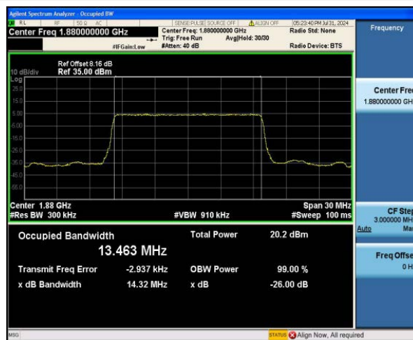
Band2-15MHz-QPSK-19125-75RB#0
