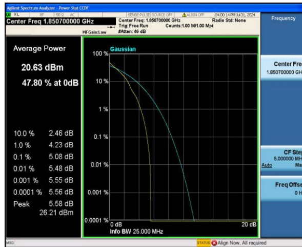
Band2-1.4MHz-QPSK-18607-6RB#0
