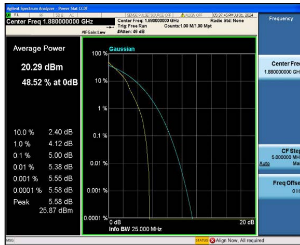
Band2-15MHz-QPSK-18900-75RB#0
