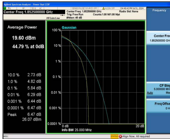
Band2-5MHz-16QAM-18625-25RB#0
