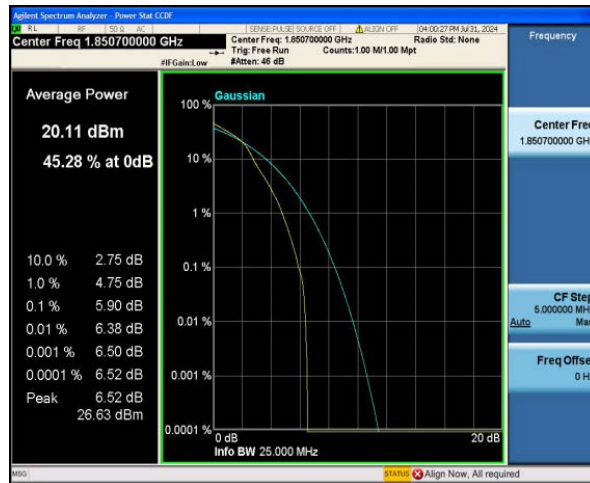
Band2-1.4MHz-16QAM-18607-6RB#0
