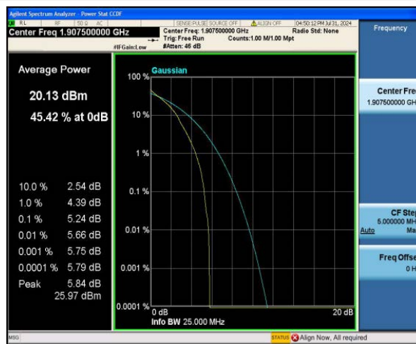
Band2-5MHz-QPSK-19175-25RB#0
