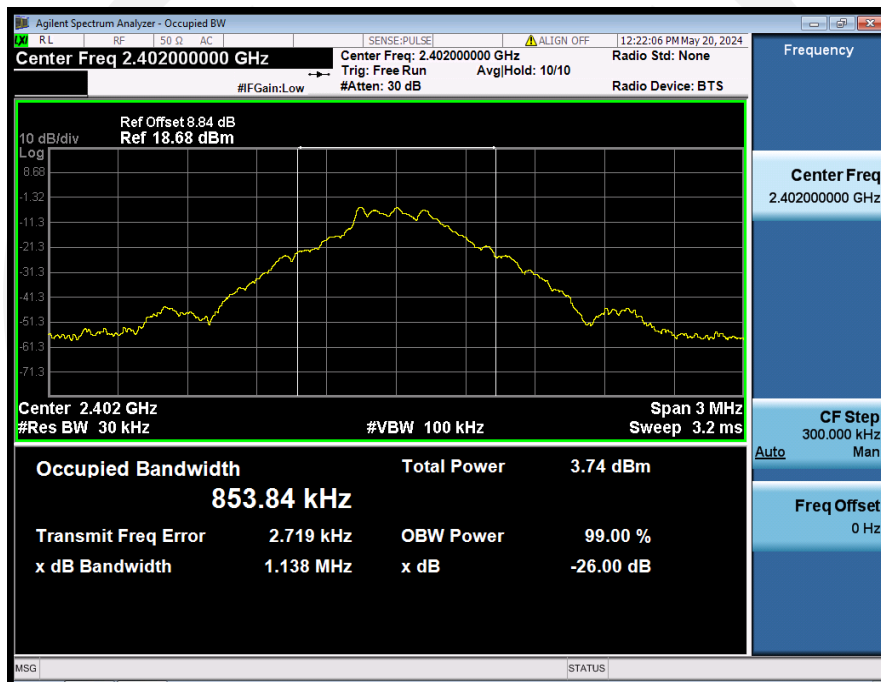
99%_Occupied_Bandwidth_NVNT_ANT1_1-DH1_2402
