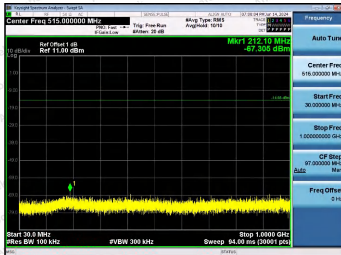
DH5-Ant1-2402-30~1000-PASS
