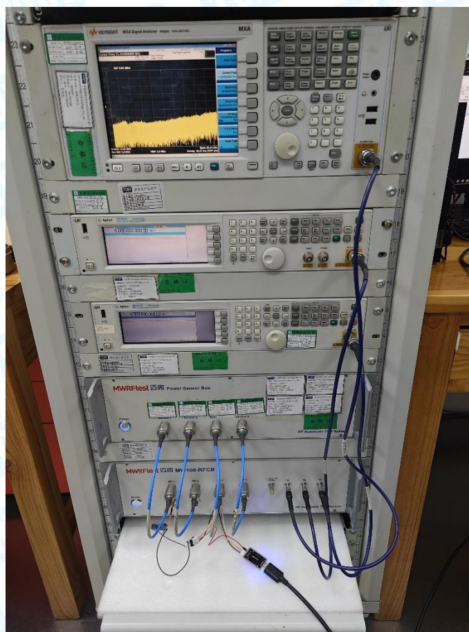
Photo of Conducted Measurements Test
