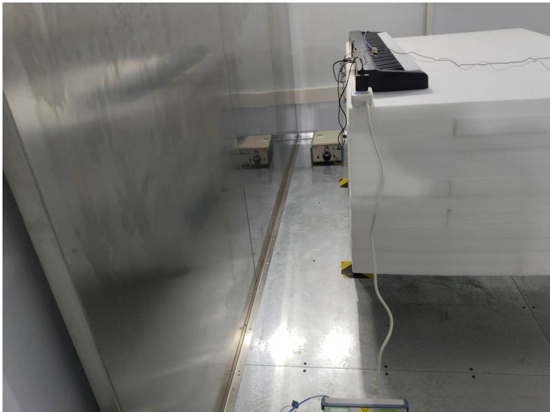
CE-Rear View
