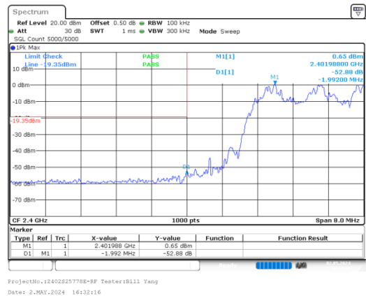
8DPSK_Hopping_Lower_3DH1
