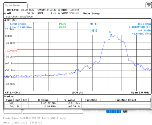
8DPSK_Low_3DH1
