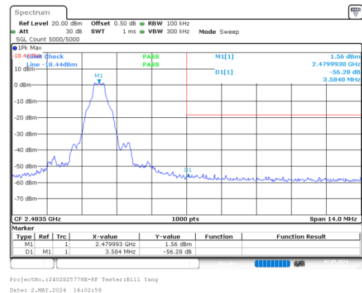
GFSK_High_DH1
