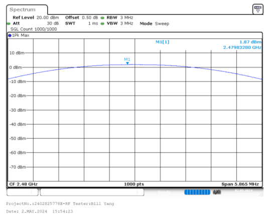
8DPSK_High_3DH1
