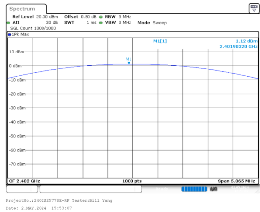
8DPSK_Low_3DH1
