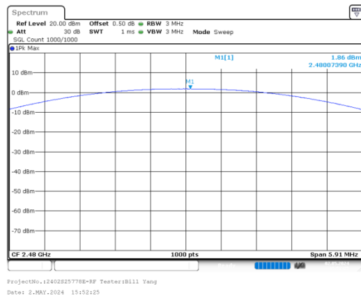
\pi/4 -DQPSK_High_2DH1
