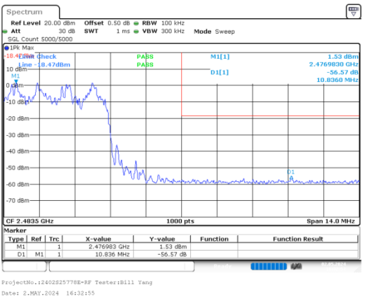
8DPSK_Hopping_Upper_3DH1
