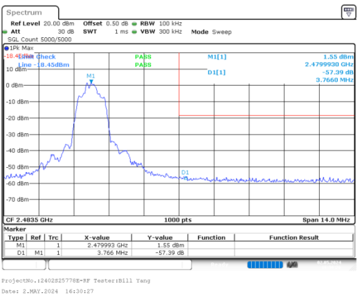
8DPSK_High_3DH1
