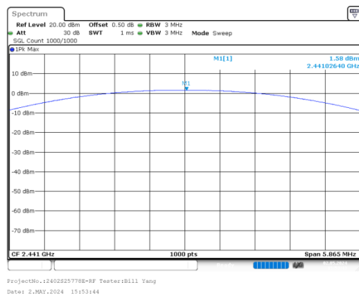
8DPSK_Mid_3DH1
