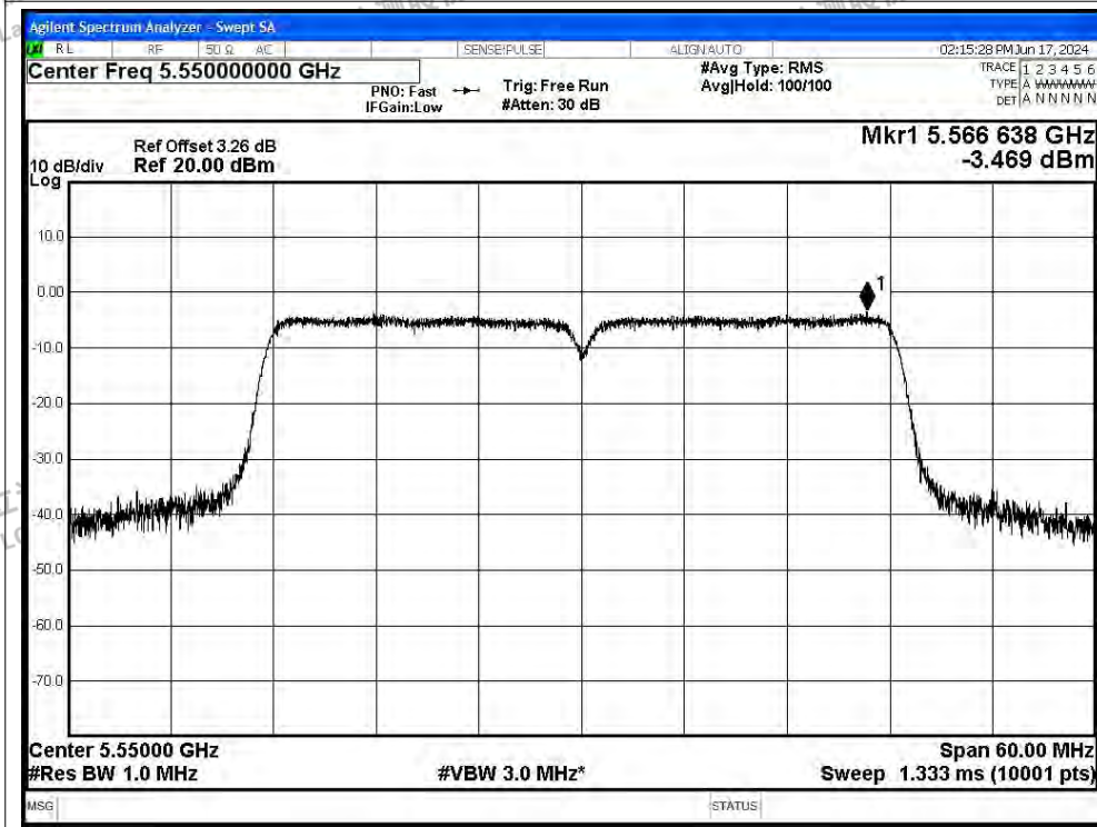
PSD NVNT n40 5550MHz Ant3
