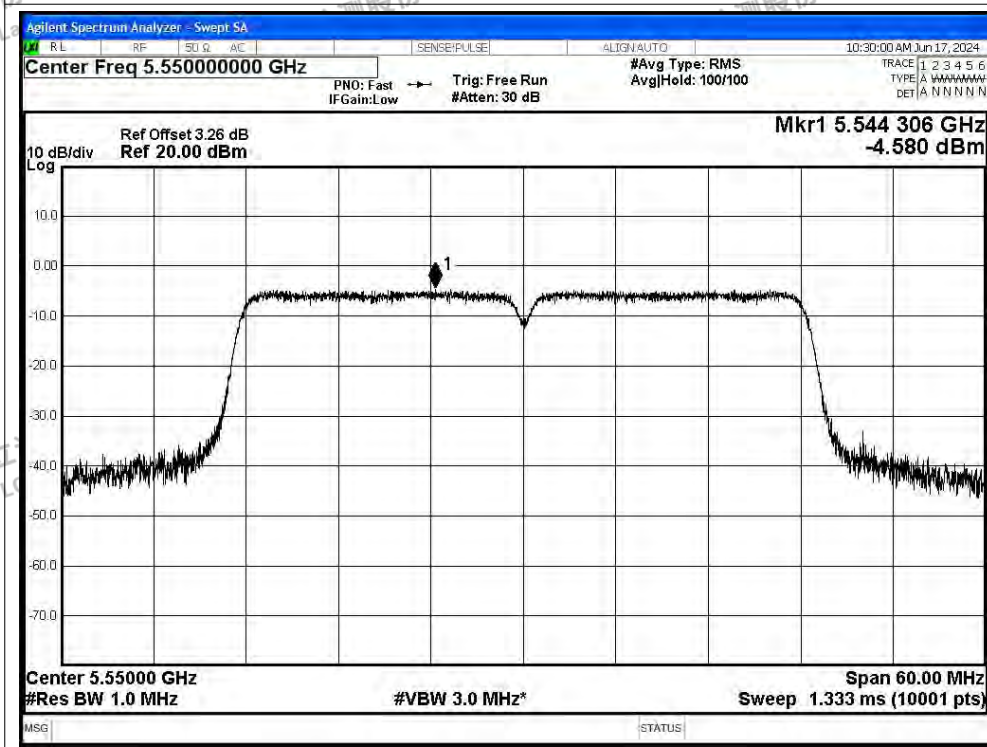
PSD NVNT n40 5550MHz Ant4
