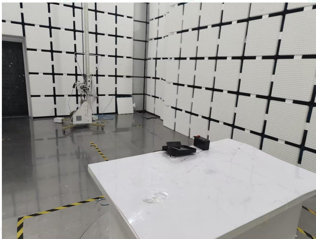
Radiated Emission below 1GHz mode
