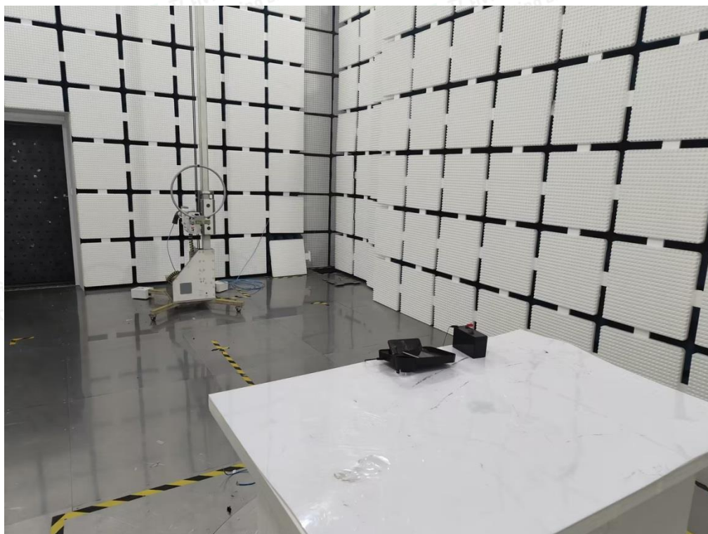
Radiated Emission below 30MHz mode
