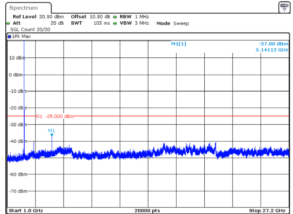
5MHz_Low_QPSK_1@0(1GHz~27.2GHz)
