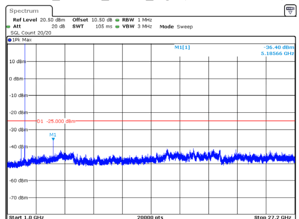
5MHz_Middle_QPSK_1@0(1GHz~27.2GHz)
