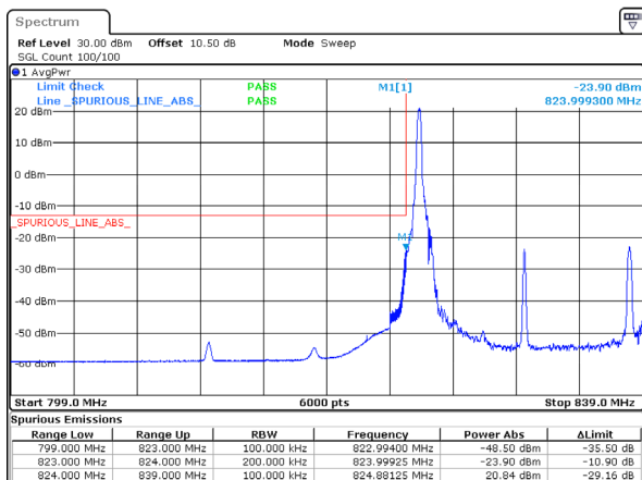
B26_2_15MHz_Low_16QAM_1@0
