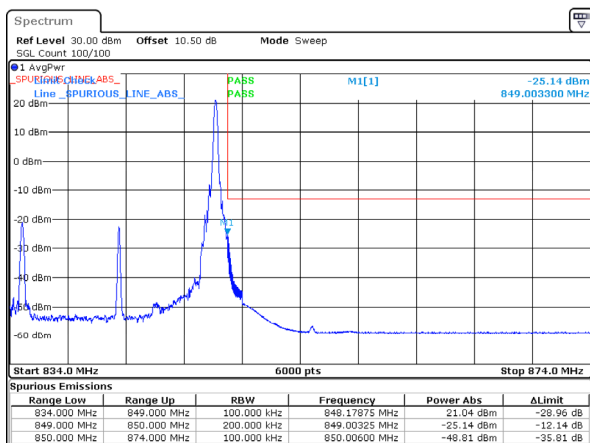
B26_2_15MHz_High_16QAM_1@74
