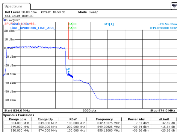
B26_2_15MHz_High_16QAM_75@0
