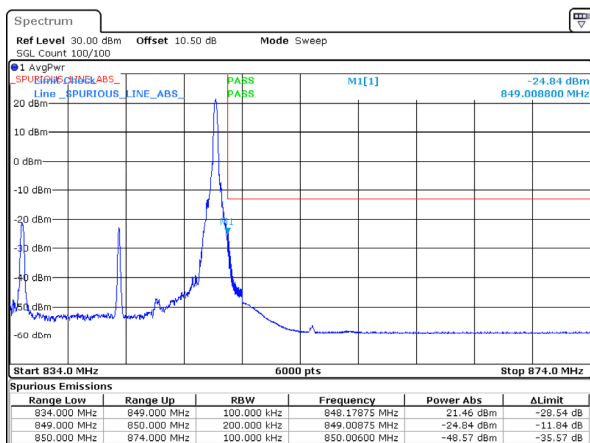
B26_2_15MHz_High_QPSK_1@74
