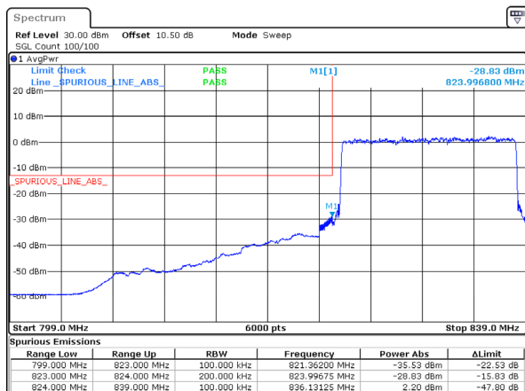
B26_2_15MHz_Low_16QAM_75@0
