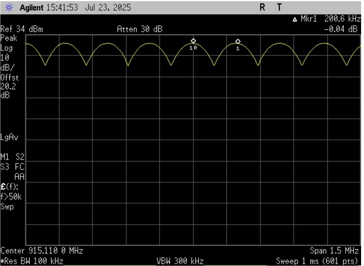
Plot 27 – Carrier Frequency Separation (Using Delta Marker Method)
