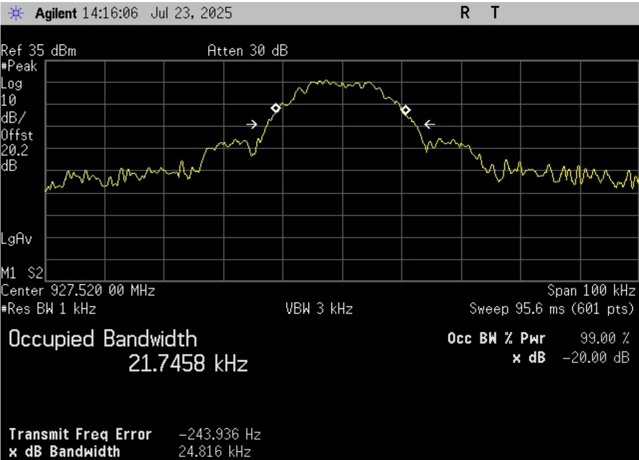
Plot 6 – Highest Channel – 20dB BW
