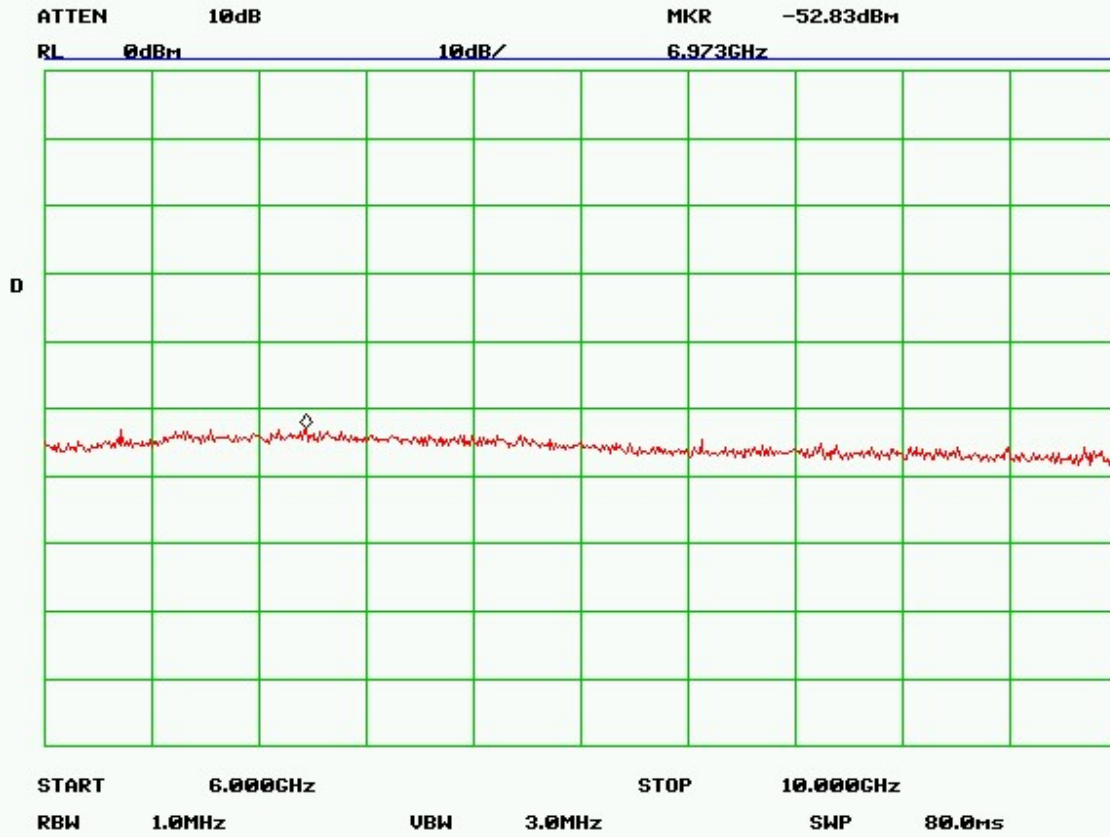
Plot 18 – High Band – 6GHz to 10GHz
