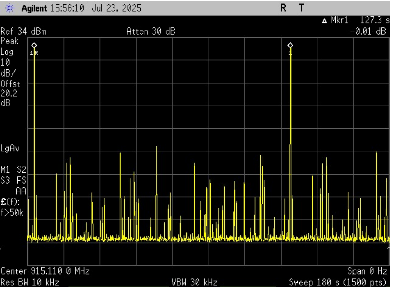
Plot 25 – Channel Occupancy
