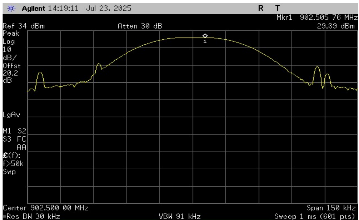
Plot 7 – Output Power – Lowest Channel
