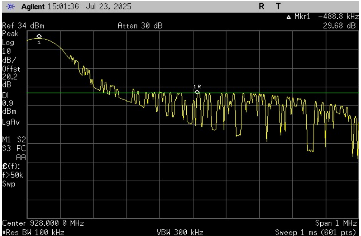
Plot 20 – Band Edge - High Channel
