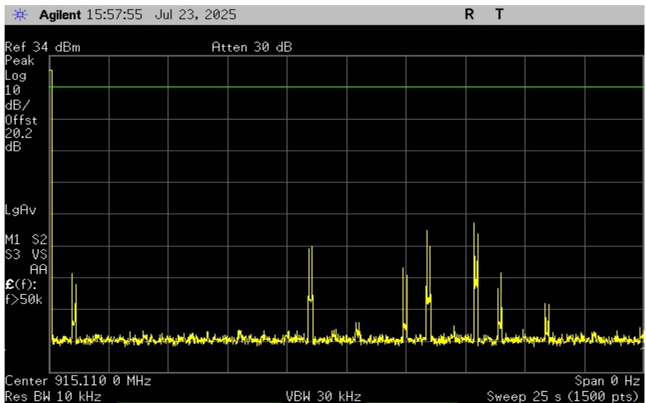
Plot 24 – Channel Occupancy
