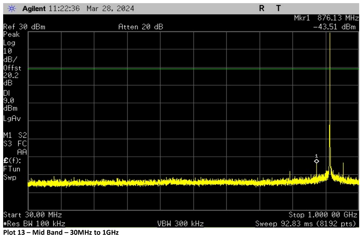
Plot 13 – Mid Band – 30MHz to 1GHz
