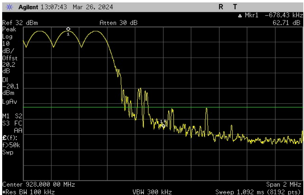
Plot 22 - Band Edge – High Channel (Hopping)
