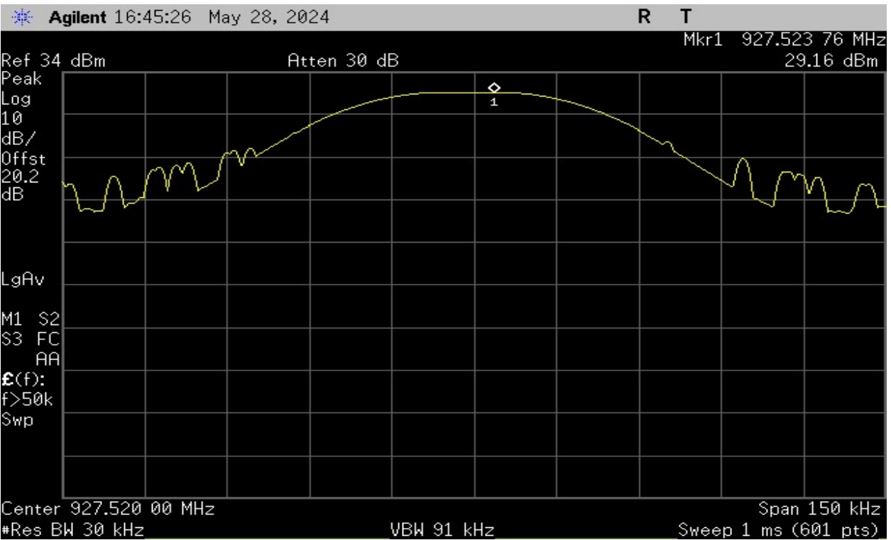
Plot 9 – Output Power – Highest Channel
