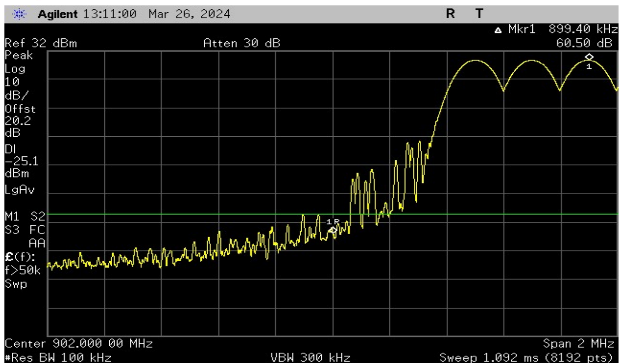
Plot 21 - Band Edge – Low Channel (Hopping)
