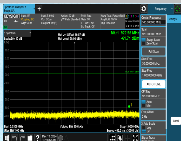
ZIGB-Ant1-2475-30~1000-PASS
