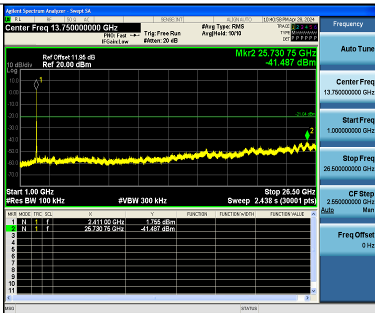
11N20SISO-Ant1-2412-1000~26500-PASS
