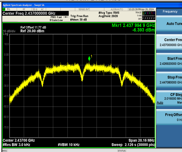
11B-Ant1-2437-PASS
