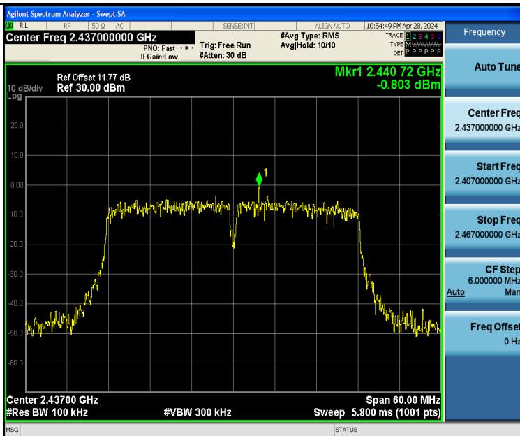
11N40SISO-Ant1-2437-0~Reference-PASS
