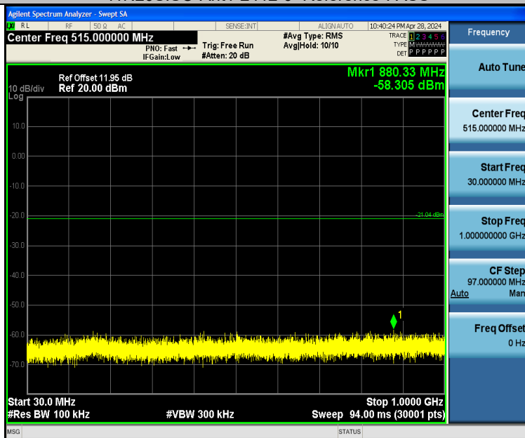
11N20SISO-Ant1-2412-30~1000-PASS
