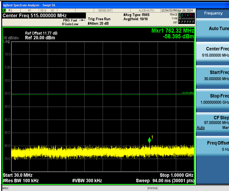
11N40SISO-Ant1-2437-30~1000-PASS
