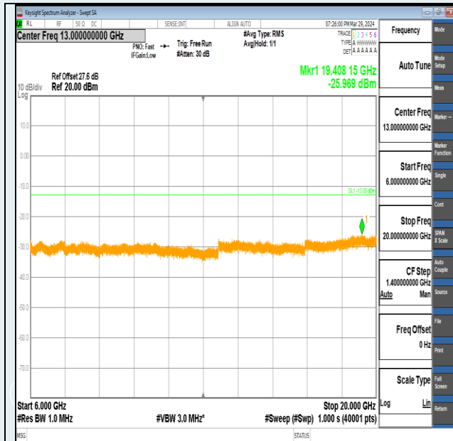
Band2-15MHz-QPSK-18900-75RB#0-6000~20000-PASS
