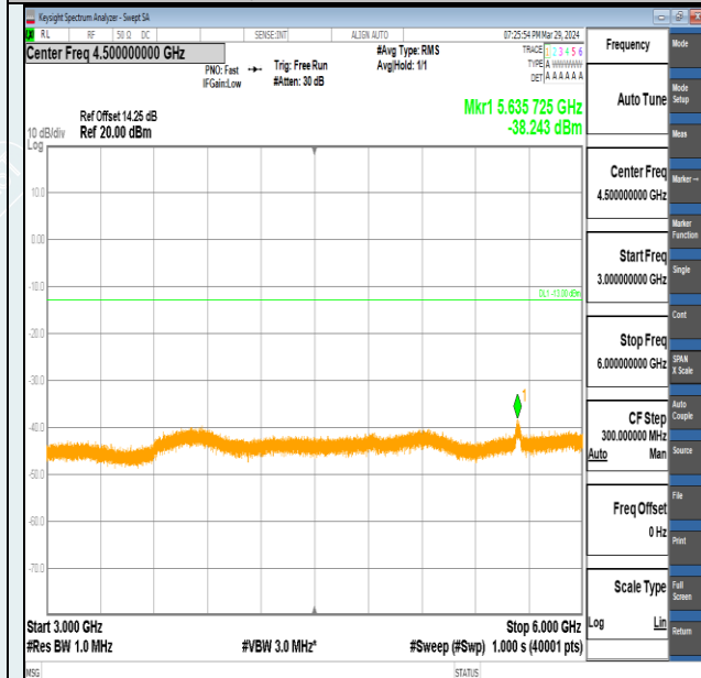
Band2-15MHz-QPSK-18900-75RB#0-3000~6000-PASS
