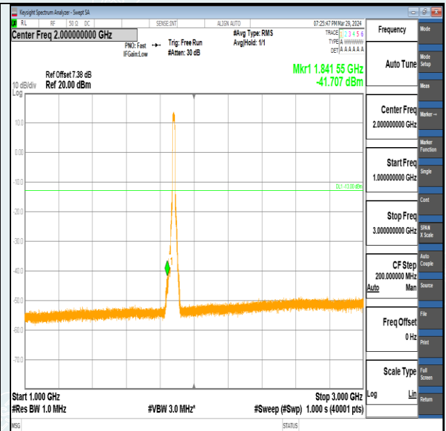
Band2-15MHz-QPSK-18900-75RB#0-1000~3000-PASS
