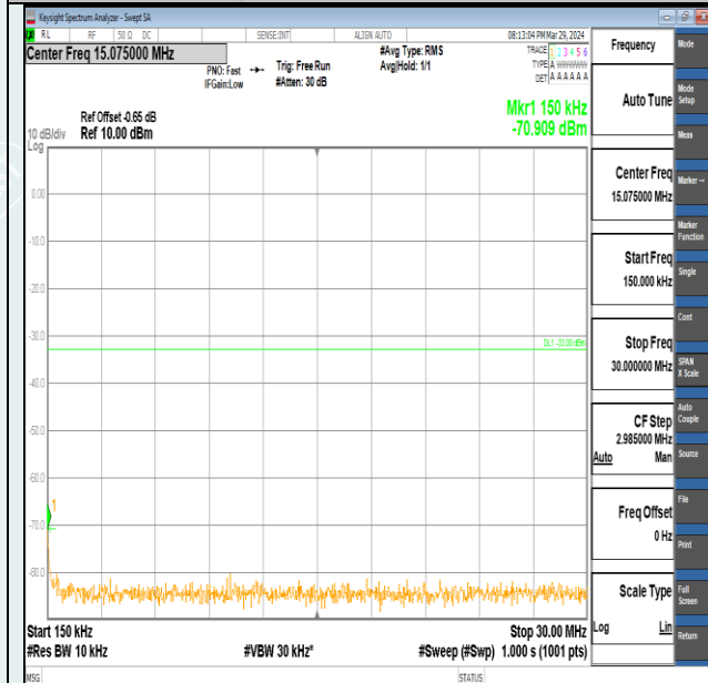
Band2-15MHz-QPSK-19125-1RB#74-0.15~30-PASS
