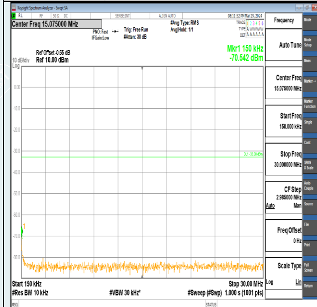
Band2-15MHz-QPSK-19125-1RB#0-0.15~30-PASS
