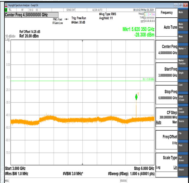
Band2-15MHz-16QAM-18900-1RB#0-3000~6000-PASS
