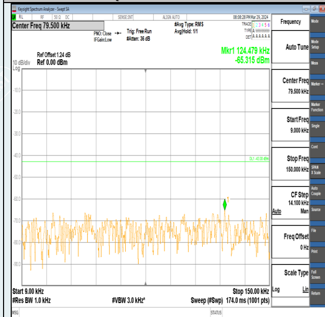
Band2-15MHz-16QAM-18675-1RB#74-0.009~0.15-PASS
