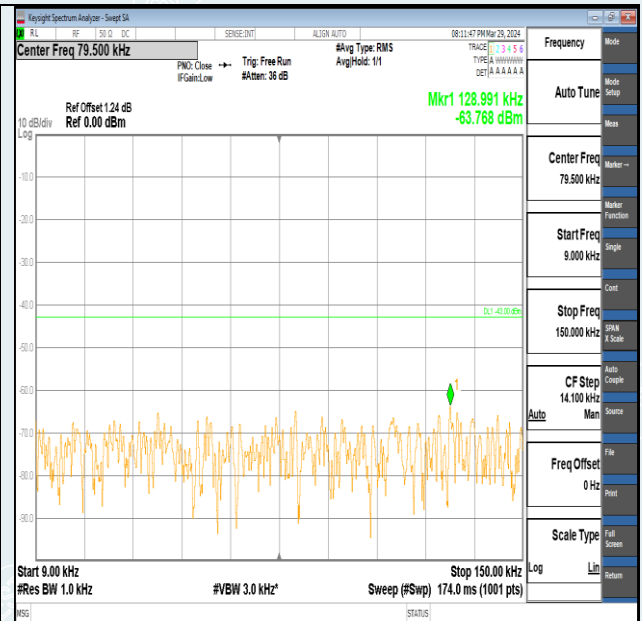
Band2-15MHz-QPSK-19125-1RB#0-0.009~0.15-PASS
