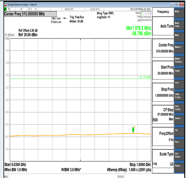
Band2-15MHz-QPSK-19125-1RB#74-30~1000-PASS
