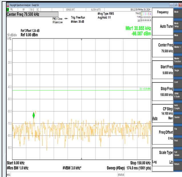
Band2-15MHz-QPSK-19125-1RB#74-0.009~0.15-PASS
