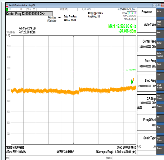
Band2-15MHz-16QAM-18675-1RB#0-6000~20000-PASS
