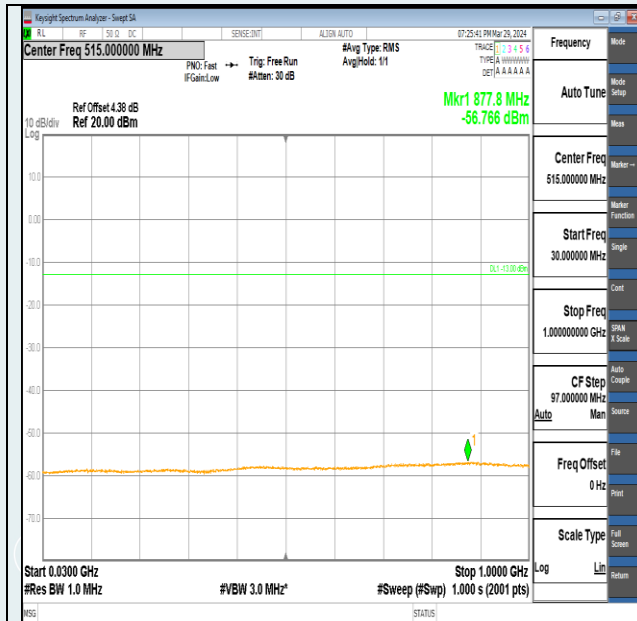
Band2-15MHz-QPSK-18900-75RB#0-30~1000-PASS
