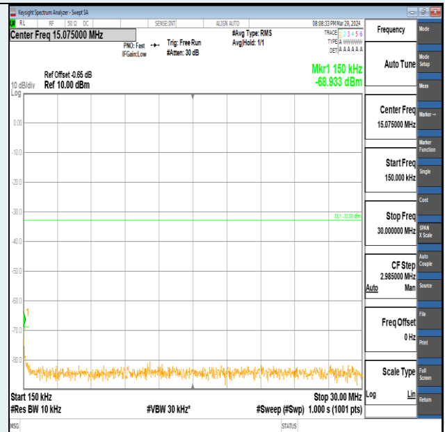
Band2-15MHz-16QAM-18675-1RB#74-0.15~30-PASS
