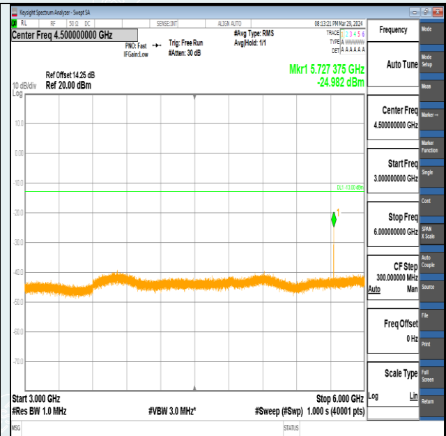
Band2-15MHz-QPSK-19125-1RB#74-3000~6000-PASS
