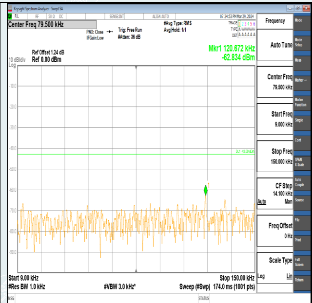
Band2-15MHz-QPSK-18675-75RB#0-0.009~0.15-PASS
