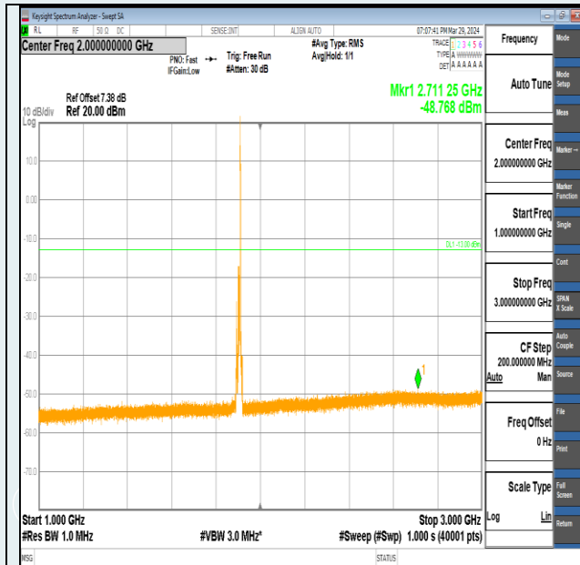
Band2-10MHz-16QAM-19150-1RB#49-1000~3000-PASS
