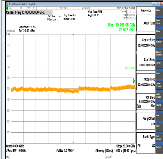
Band2-15MHz-QPSK-18900-1RB#0-6000~20000-PASS
