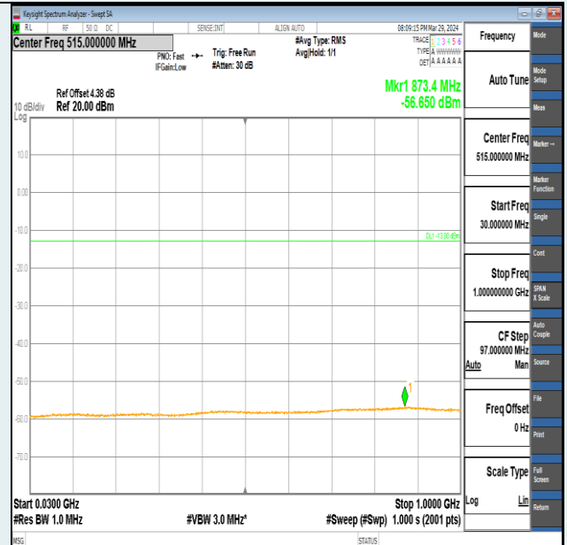
Band2-15MHz-QPSK-18900-1RB#0-30~1000-PASS
