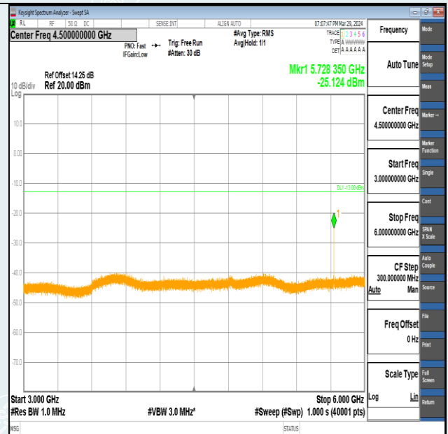
Band2-10MHz-16QAM-19150-1RB#49-3000~6000-PASS
