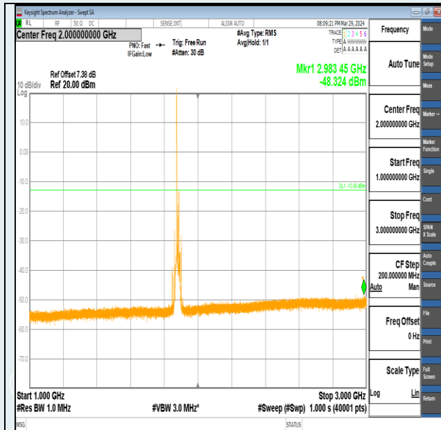
Band2-15MHz-QPSK-18900-1RB#0-1000~3000-PASS
