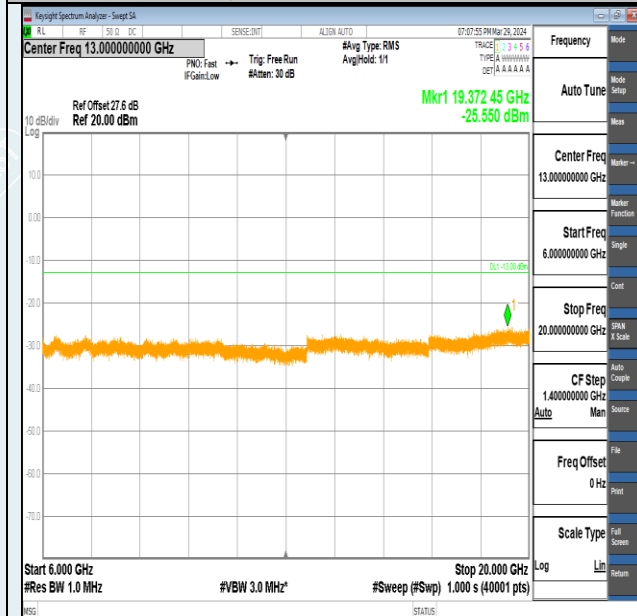
Band2-10MHz-16QAM-19150-1RB#49-6000~20000-PASS
