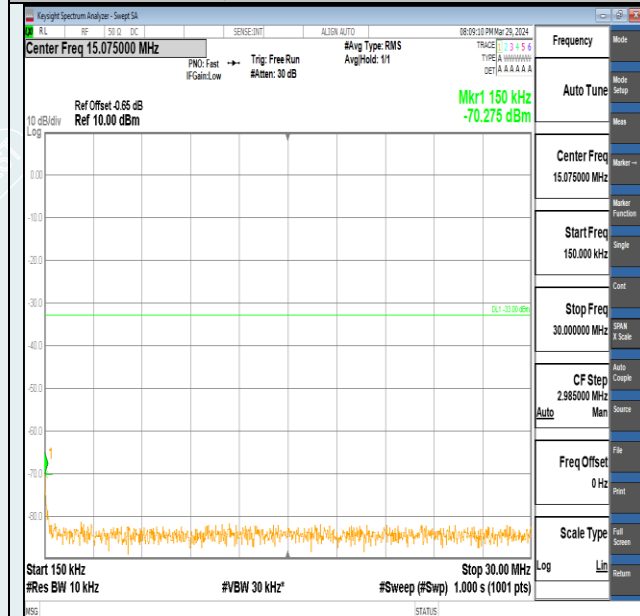
Band2-15MHz-QPSK-18900-1RB#0-0.15~30-PASS
