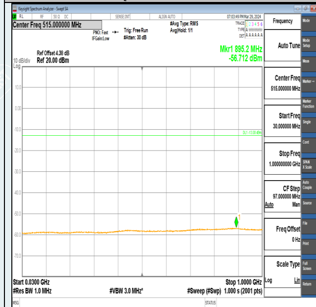
Band2-10MHz-16QAM-18900-1RB#0-30~1000-PASS
