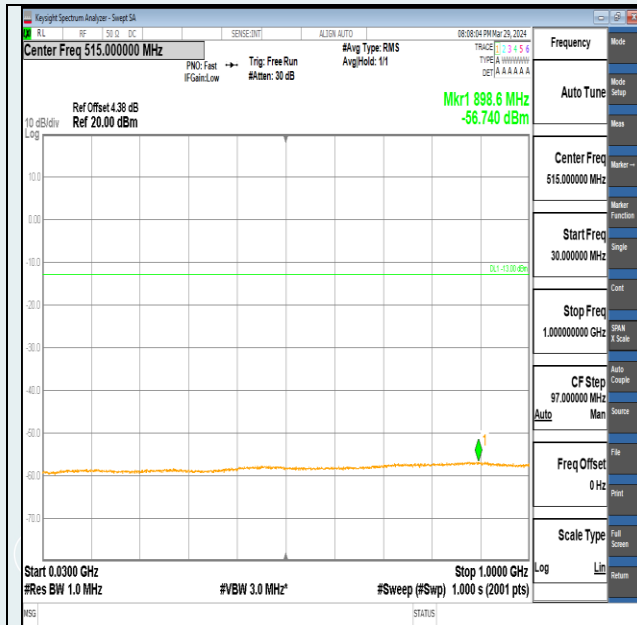
Band2-15MHz-QPSK-18675-1RB#74-30~1000-PASS
