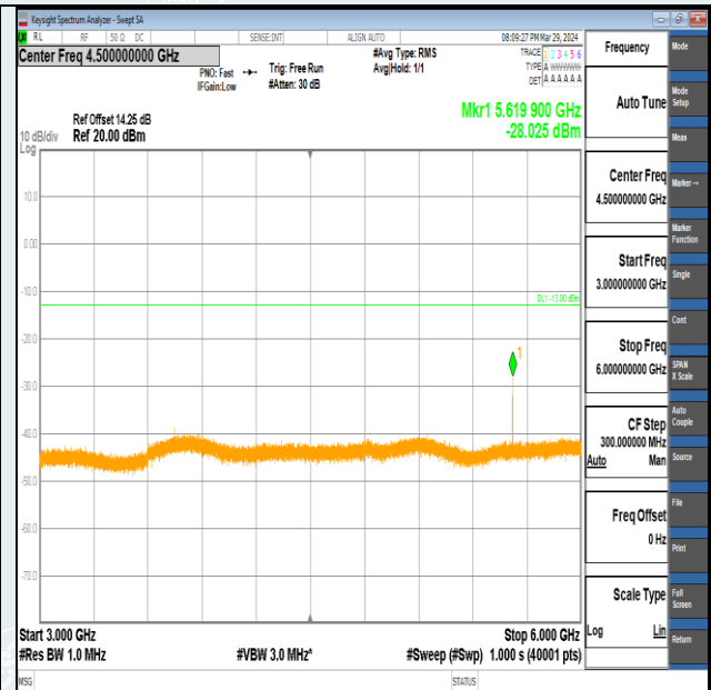
Band2-15MHz-QPSK-18900-1RB#0-3000~6000-PASS
