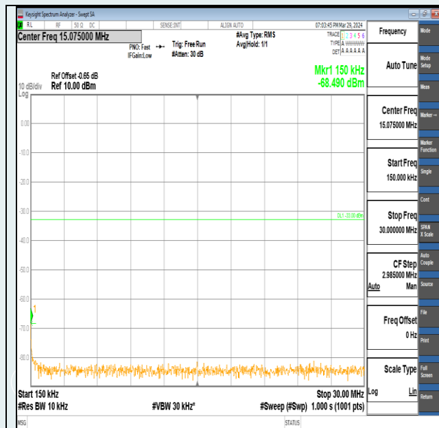
Band2-10MHz-16QAM-18900-1RB#0-0.15~30-PASS
