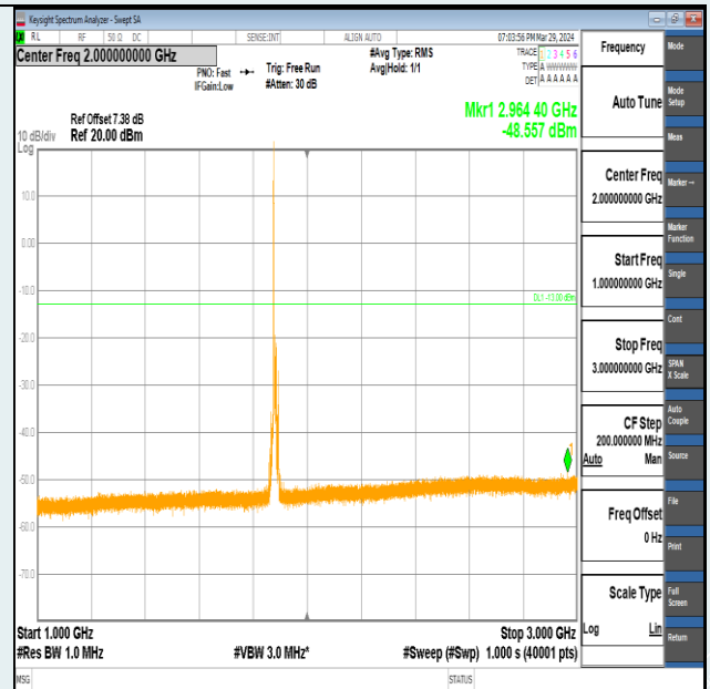
Band2-10MHz-16QAM-18900-1RB#0-1000~3000-PASS
