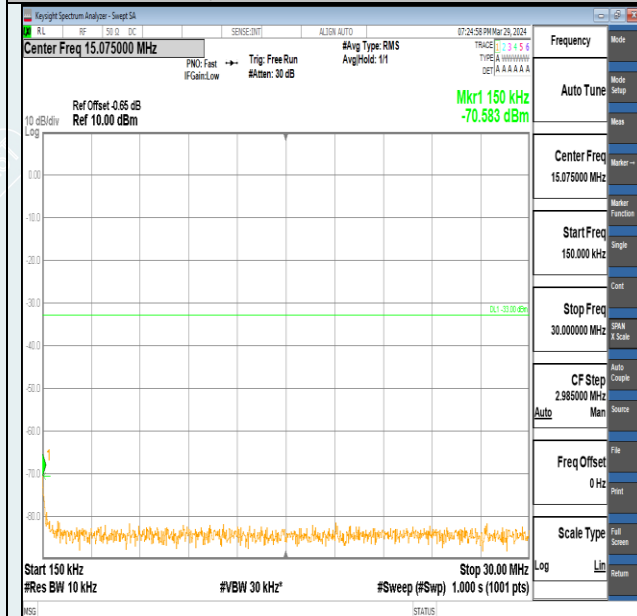
Band2-15MHz-QPSK-18675-75RB#0-0.15~30-PASS
