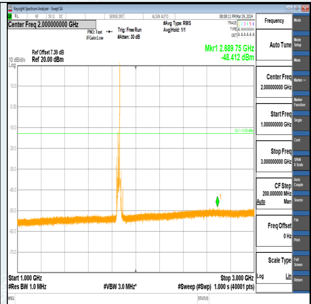
Band2-15MHz-QPSK-18675-1RB#74-1000~3000-PASS
