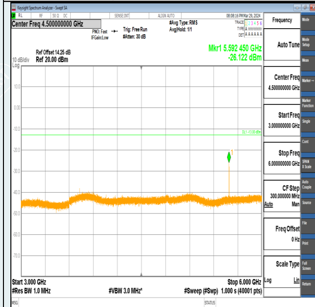
Band2-15MHz-QPSK-18675-1RB#74-3000~6000-PASS
