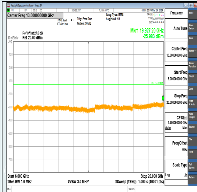
Band2-15MHz-QPSK-18675-1RB#74-6000~20000-PASS
