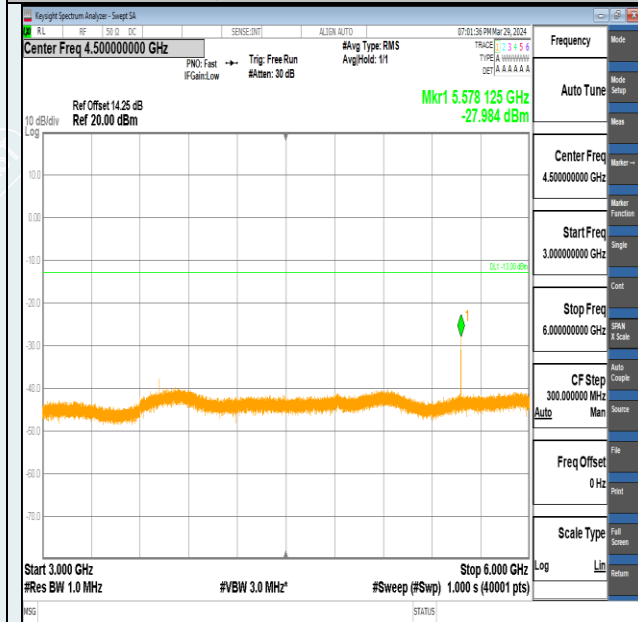
Band2-10MHz-QPSK-18650-1RB#49-3000~6000-PASS
