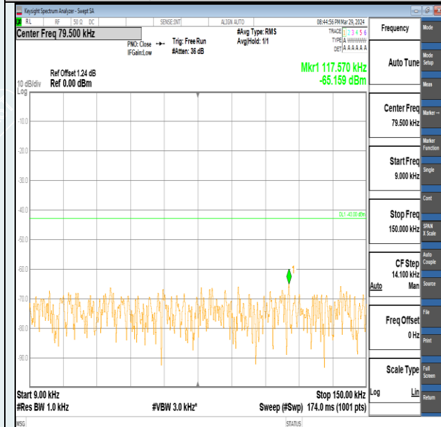
Band2-10MHz-QPSK-19150-50RB#0-0.009~0.15-PASS
