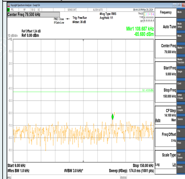
Band2-10MHz-QPSK-18900-50RB#0-0.009~0.15-PASS
