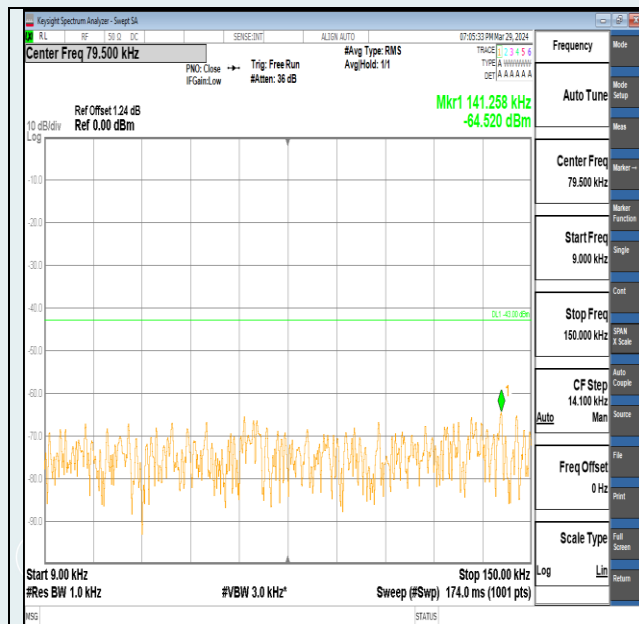
Band2-10MHz-QPSK-19150-1RB#0-0.009~0.15-PASS
