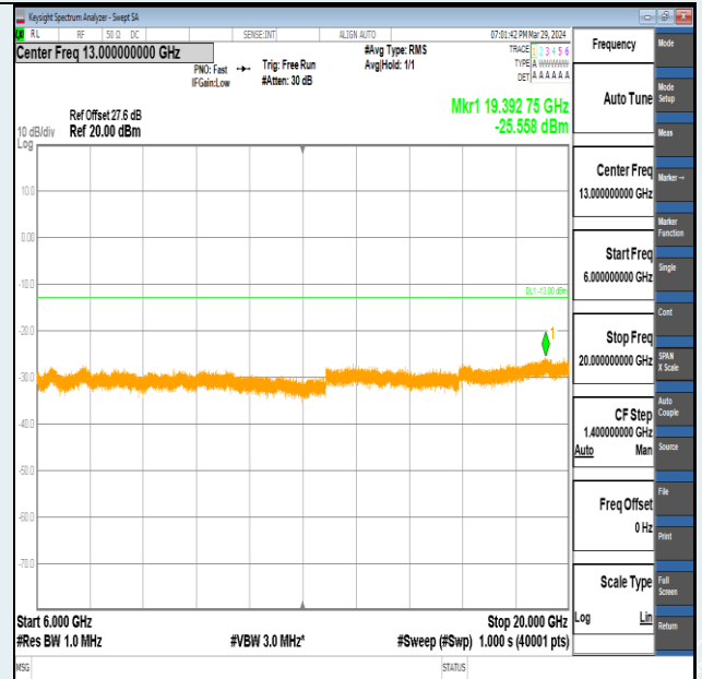
Band2-10MHz-QPSK-18650-1RB#49-6000~20000-PASS
