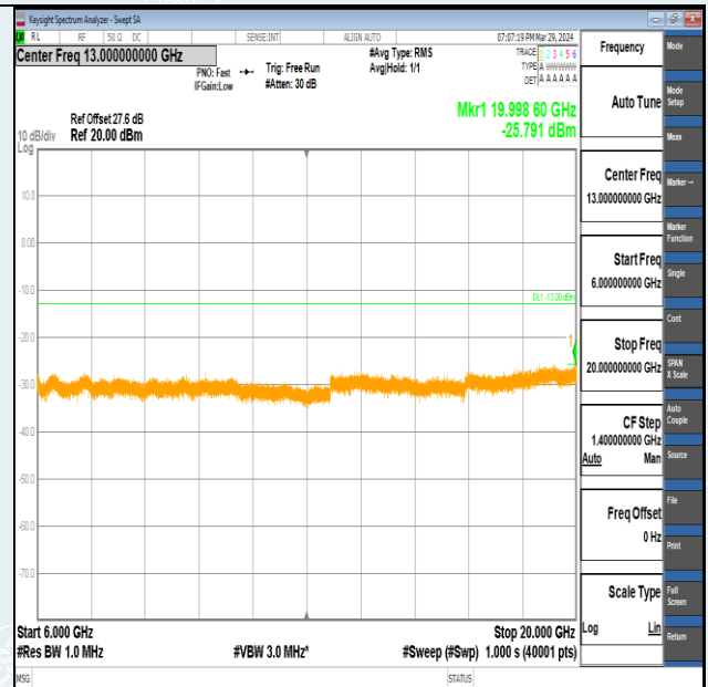
Band2-10MHz-QPSK-19150-1RB#49-6000~20000-PASS
