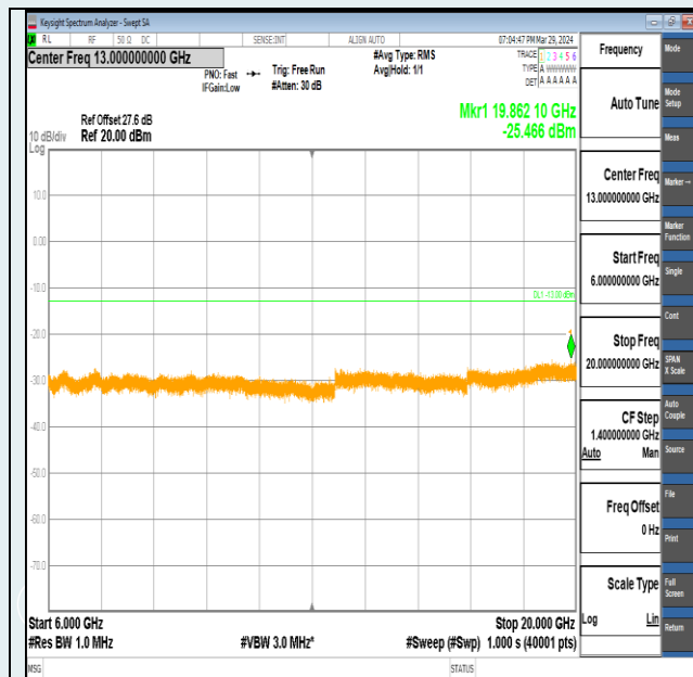
Band2-10MHz-QPSK-18900-1RB#49-6000~20000-PASS
