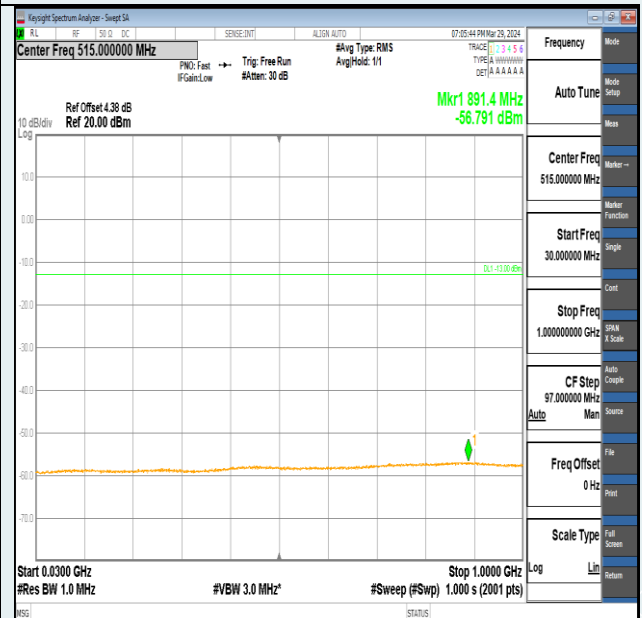
Band2-10MHz-QPSK-19150-1RB#0-30~1000-PASS
