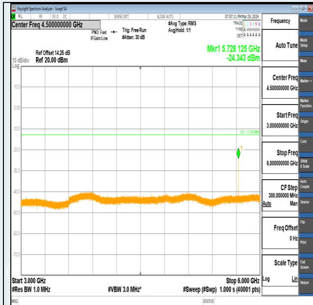
Band2-10MHz-QPSK-19150-1RB#49-3000~6000-PASS
