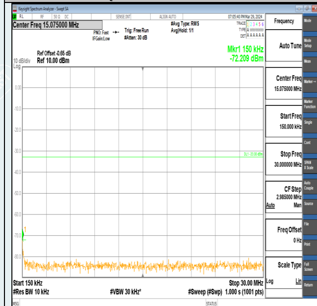
Band2-10MHz-QPSK-19150-1RB#0-0.15~30-PASS
