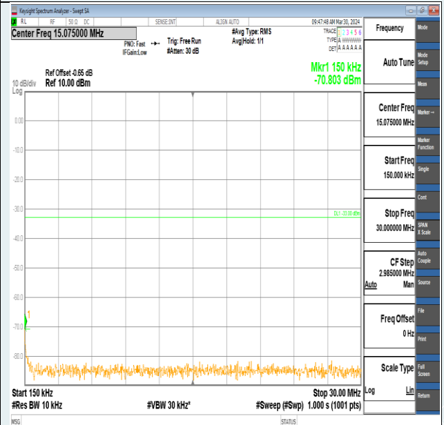
Band2-5MHz-16QAM-19175-1RB#0-0.15~30-PASS
