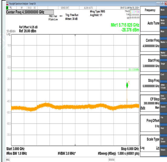
Band2-5MHz-QPSK-19175-1RB#0-3000~6000-PASS
