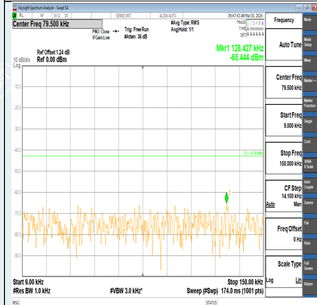
Band2-5MHz-16QAM-19175-1RB#0-0.009~0.15-PASS
