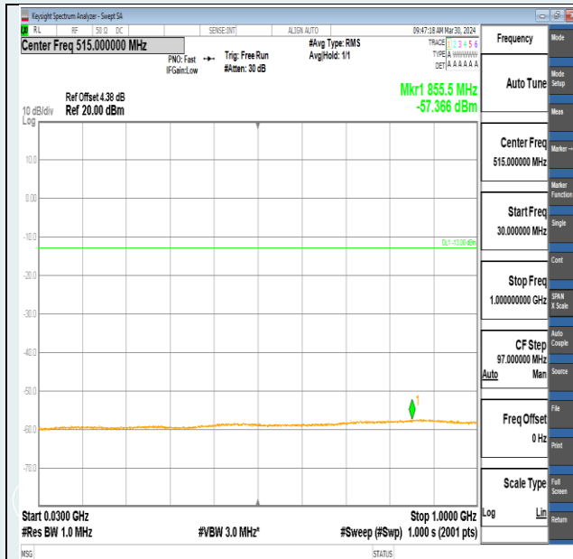
Band2-5MHz-QPSK-19175-1RB#0-30~1000-PASS
