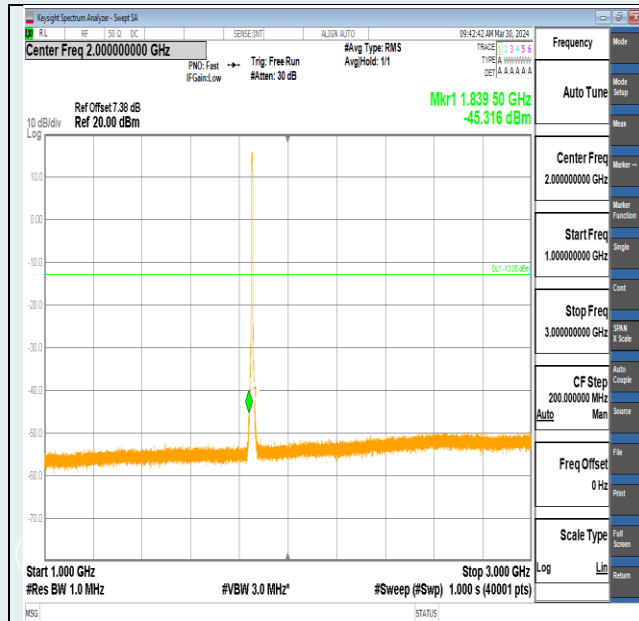
Band2-5MHz-16QAM-18625-25RB#0-1000~3000-PASS
