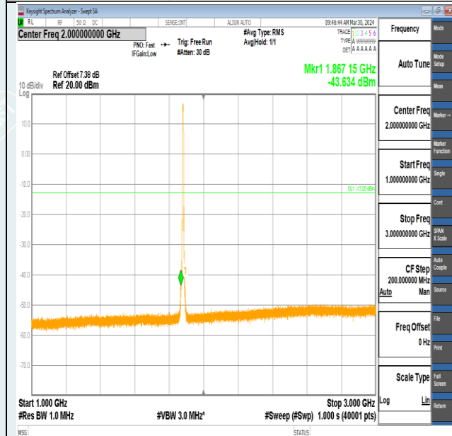
Band2-5MHz-16QAM-18900-25RB#0-1000~3000-PASS
