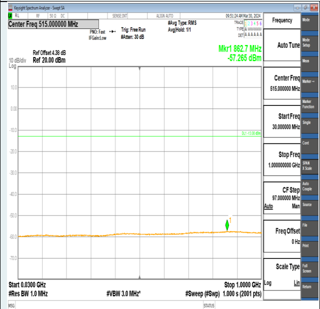
Band2-5MHz-QPSK-19175-25RB#0-30~1000-PASS
