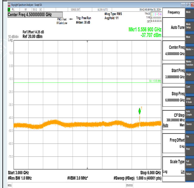
Band2-5MHz-16QAM-18625-25RB#0-3000~6000-PASS
