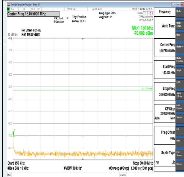
Band2-5MHz-QPSK-19175-25RB#0-0.15~30-PASS
