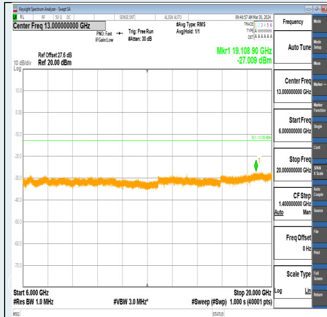
Band2-5MHz-16QAM-18900-25RB#0-6000~20000-PASS
