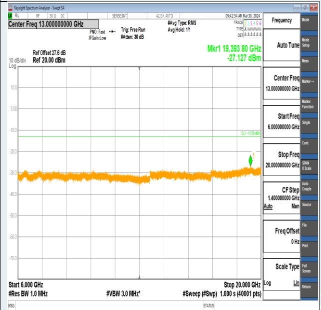
Band2-5MHz-16QAM-18625-25RB#0-6000~20000-PASS
