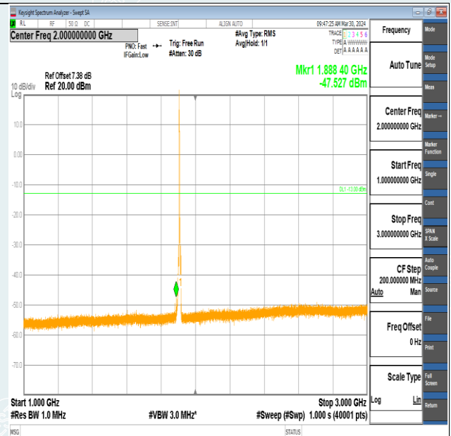
Band2-5MHz-QPSK-19175-1RB#0-1000~3000-PASS
