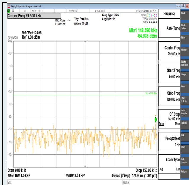
Band2-5MHz-QPSK-19175-25RB#0-0.009~0.15-PASS
