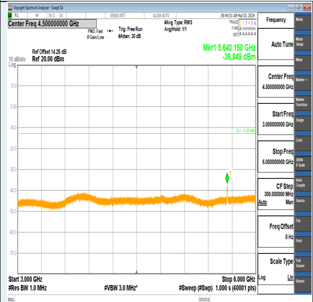
Band2-5MHz-16QAM-18900-25RB#0-3000~6000-PASS
