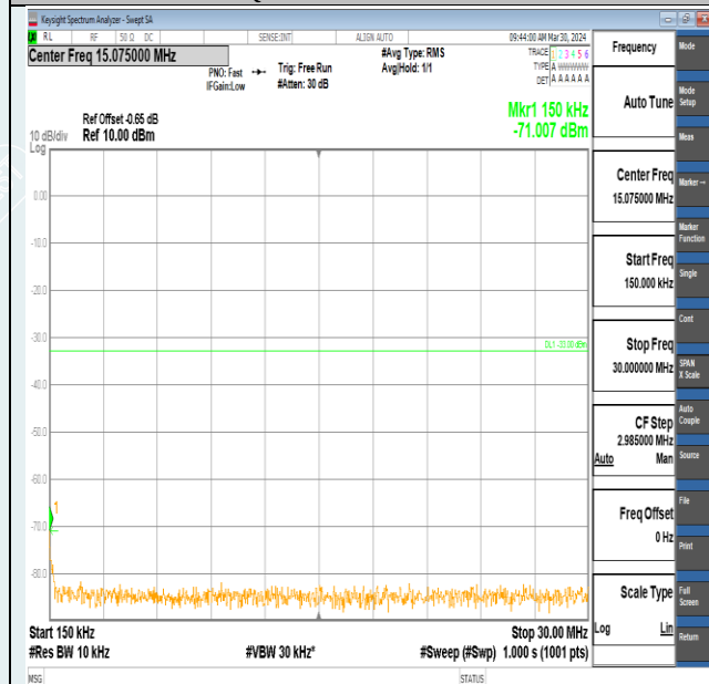
Band2-5MHz-16QAM-18900-1RB#0-0.15~30-PASS
