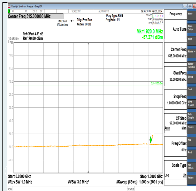
Band2-5MHz-16QAM-18900-25RB#0-30~1000-PASS
