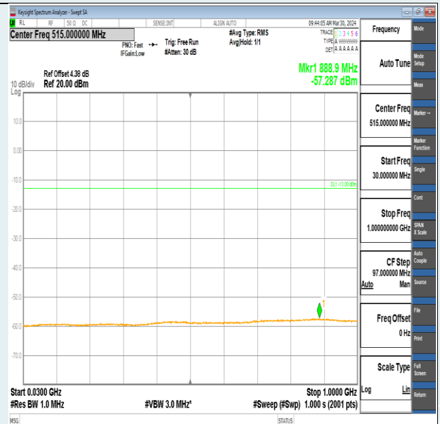
Band2-5MHz-16QAM-18900-1RB#0-30~1000-PASS
