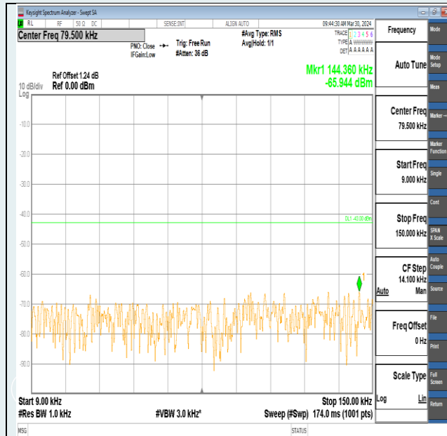
Band2-5MHz-QPSK-18900-1RB#24-0.009~0.15-PASS
