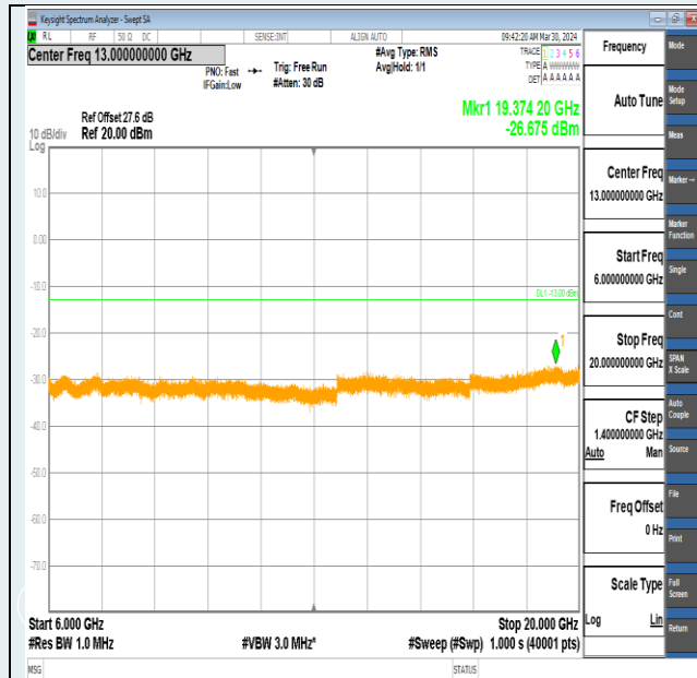
Band2-5MHz-QPSK-18625-25RB#0-6000~20000-PASS
