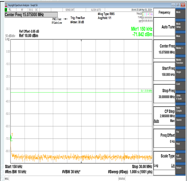
Band2-5MHz-QPSK-18900-1RB#24-0.15~30-PASS
