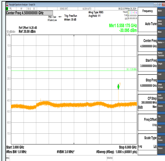
Band2-3MHz-16QAM-18615-1RB#14-3000~6000-PASS
