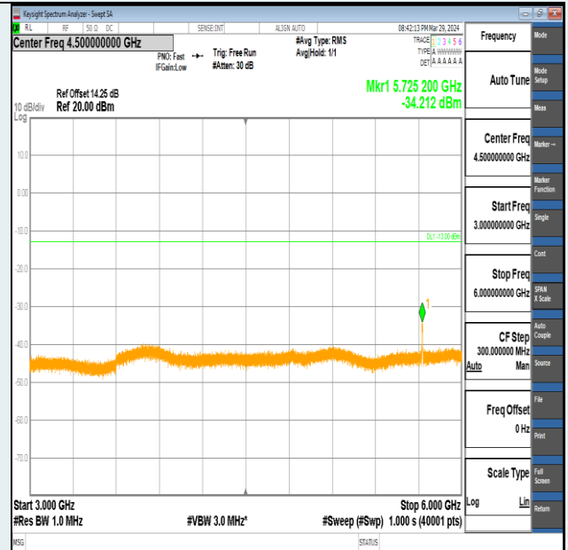
Band2-3MHz-QPSK-19185-15RB#0-3000~6000-PASS
