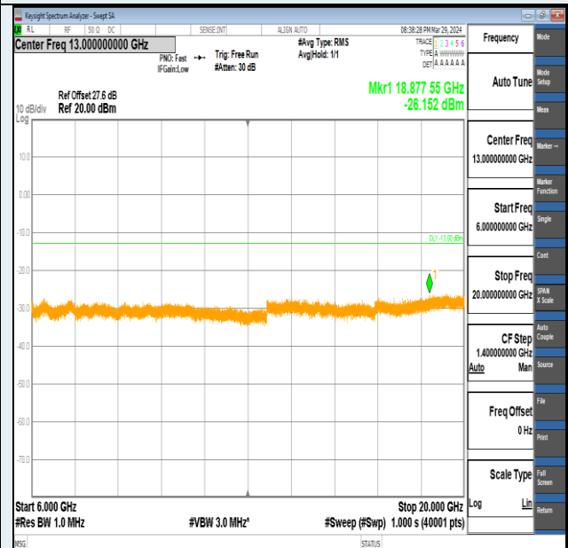
Band2-3MHz-QPSK-18900-15RB#0-6000~20000-PASS
