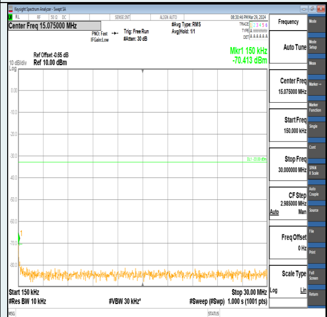
Band2-3MHz-16QAM-18615-1RB#0-0.15~30-PASS
