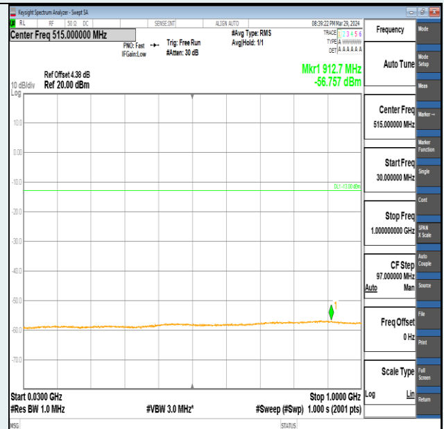
Band2-3MHz-QPSK-19185-1RB#0-30~1000-PASS
