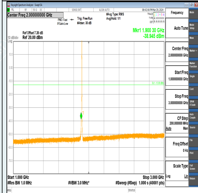
Band2-3MHz-QPSK-19185-15RB#0-1000~3000-PASS
