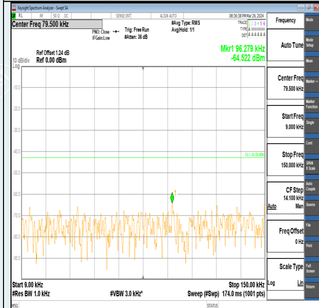
Band2-3MHz-QPSK-18900-1RB#14-0.009~0.15-PASS
