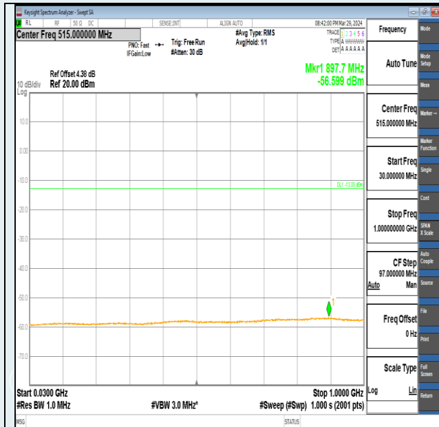
Band2-3MHz-QPSK-19185-15RB#0-30~1000-PASS
