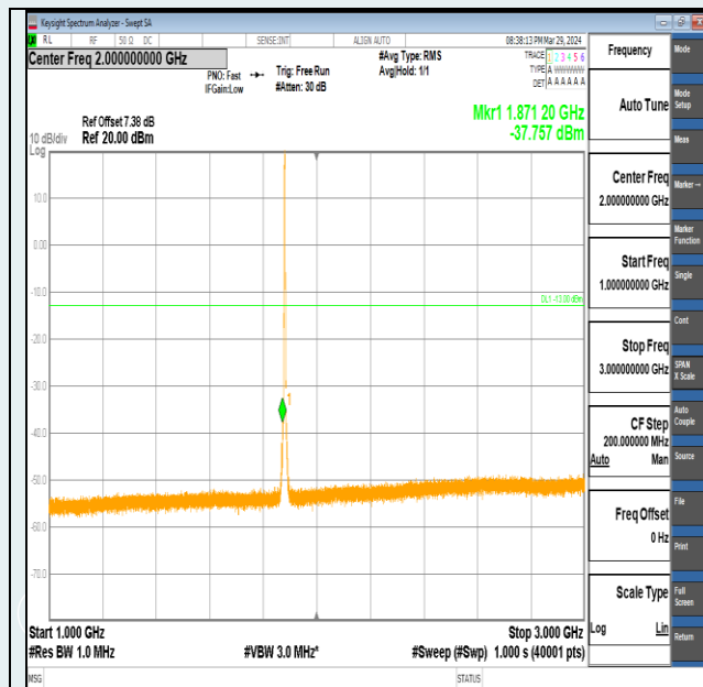
Band2-3MHz-QPSK-18900-15RB#0-1000~3000-PASS
