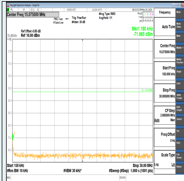
Band2-3MHz-QPSK-18900-1RB#0-0.15~30-PASS
