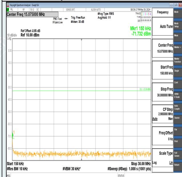
Band2-3MHz-QPSK-19185-1RB#0-0.15~30-PASS
