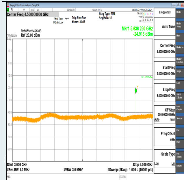
Band2-3MHz-QPSK-18900-1RB#0-3000~6000-PASS
