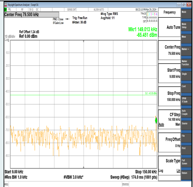
Band2-3MHz-16QAM-18615-15RB#0-0.009~0.15-PASS
