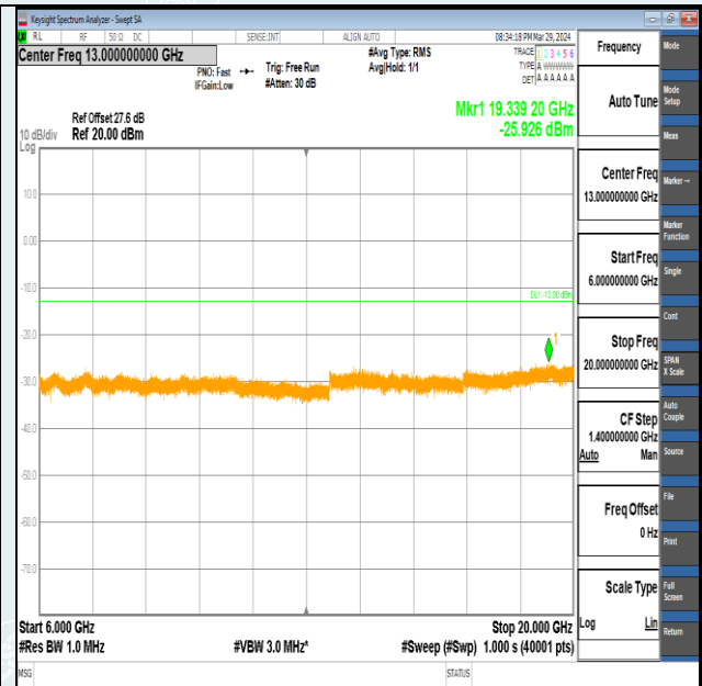
Band2-3MHz-QPSK-18900-1RB#0-6000~20000-PASS
