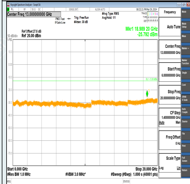
Band2-3MHz-16QAM-18615-1RB#14-6000~20000-PASS
