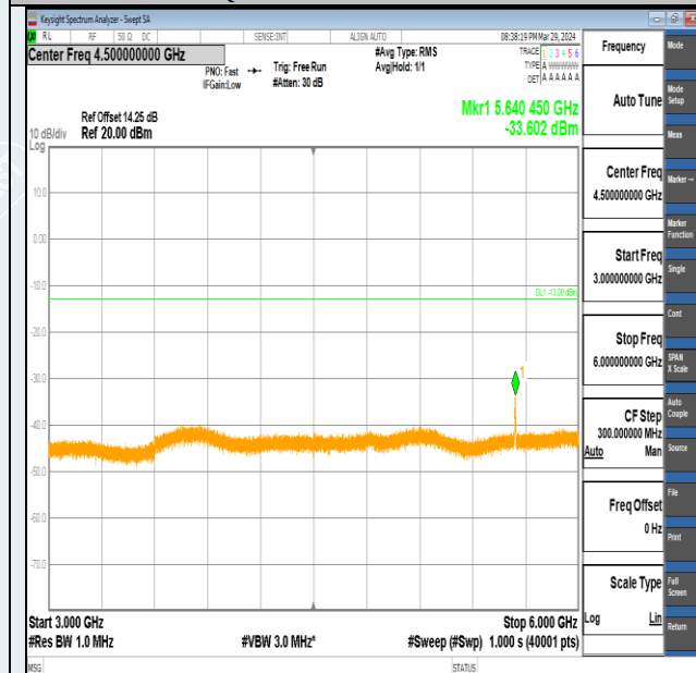
Band2-3MHz-QPSK-18900-15RB#0-3000~6000-PASS
