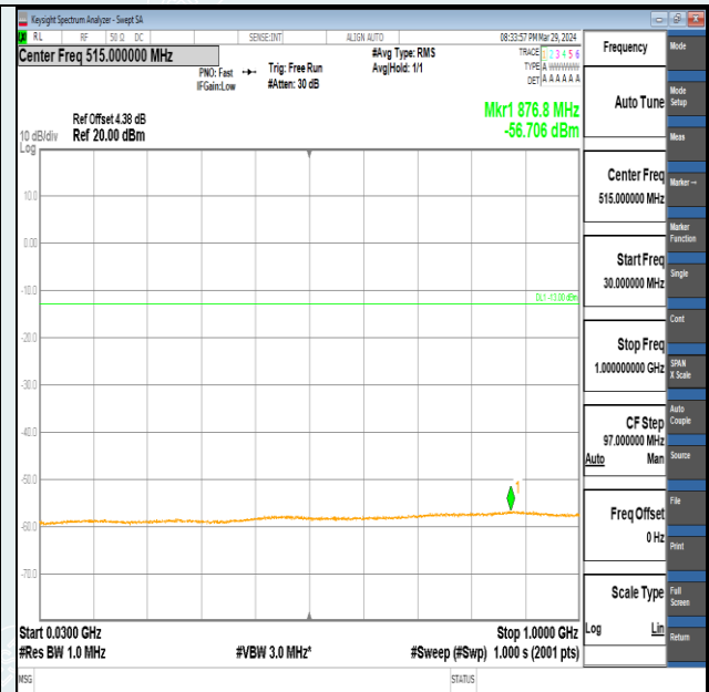
Band2-3MHz-QPSK-18900-1RB#0-30~1000-PASS
