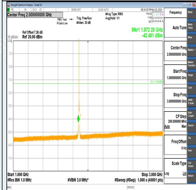
Band2-3MHz-QPSK-18900-1RB#0-1000~3000-PASS
