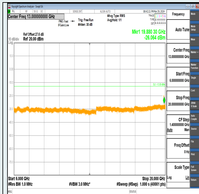
Band2-3MHz-QPSK-19185-15RB#0-6000~20000-PASS
