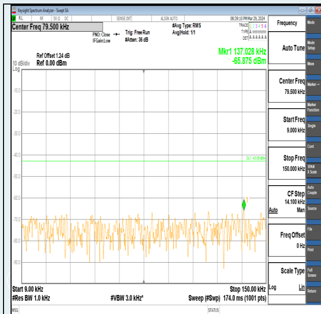
Band2-3MHz-QPSK-19185-1RB#0-0.009~0.15-PASS
