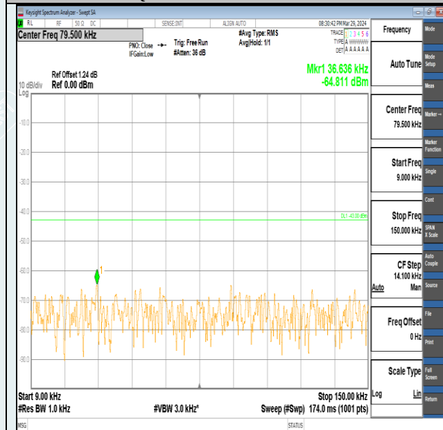
Band2-3MHz-16QAM-18615-1RB#0-0.009~0.15-PASS
