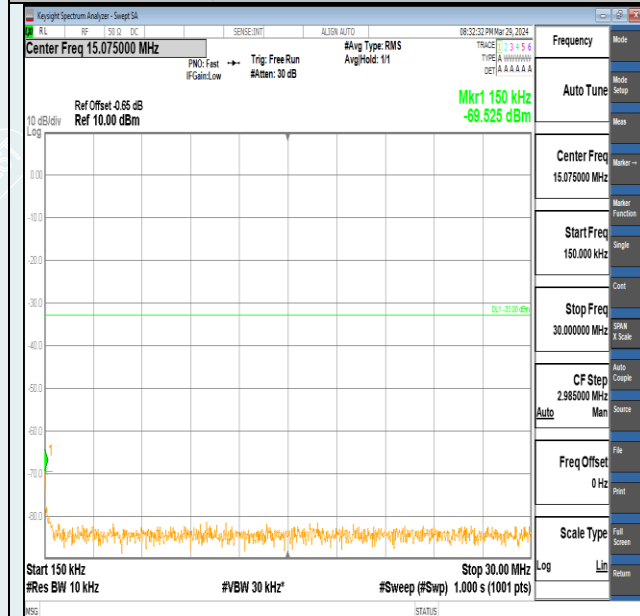
Band2-3MHz-QPSK-18615-15RB#0-0.15~30-PASS
