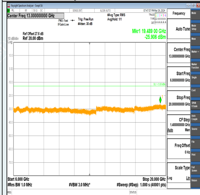
Band2-1.4MHz-16QAM-18900-1RB#0-6000~20000-PASS
