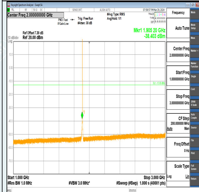
Band2-1.4MHz-16QAM-19193-6RB#0-1000~3000-PASS
