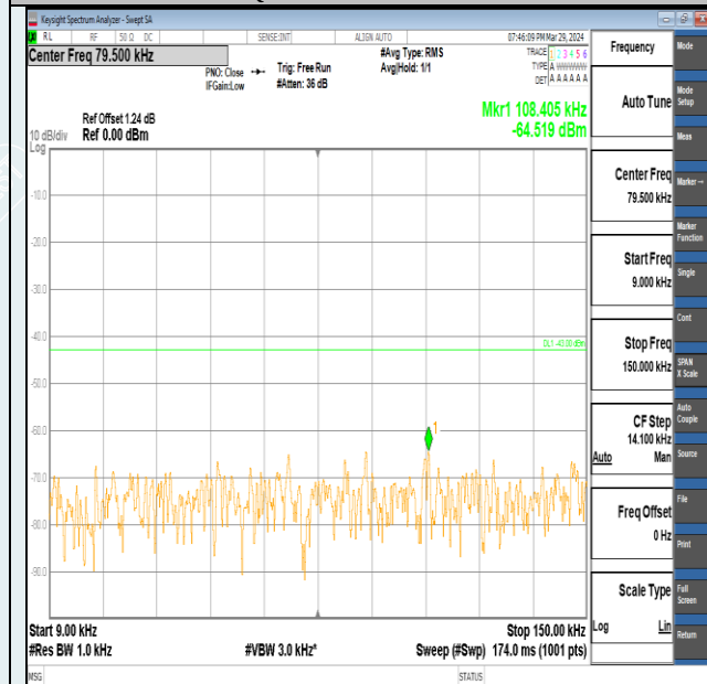
Band2-1.4MHz-16QAM-18607-6RB#0-0.009~0.15-PASS
