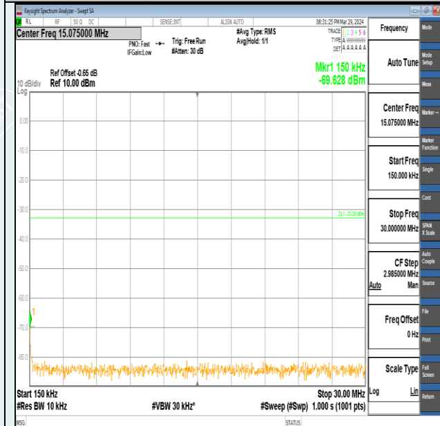
Band2-3MHz-QPSK-18615-1RB#14-0.15~30-PASS
