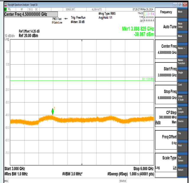
Band2-1.4MHz-16QAM-18607-1RB#5-3000~6000-PASS
