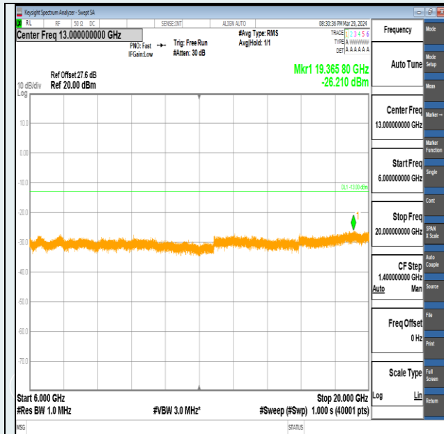
Band2-3MHz-QPSK-18615-1RB#0-6000~20000-PASS
