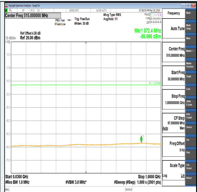
Band2-1.4MHz-16QAM-19193-6RB#0-30~1000-PASS
