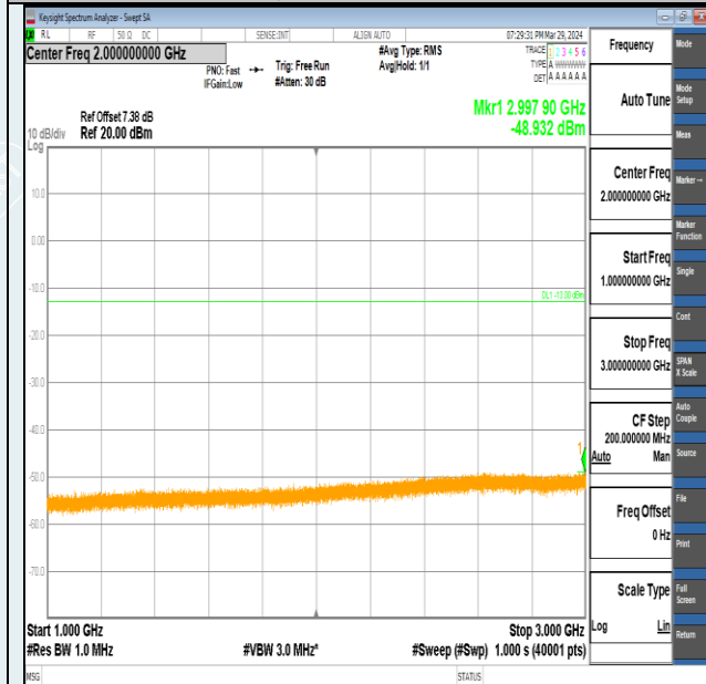
Band2-1.4MHz-16QAM-18607-1RB#5-1000~3000-PASS
