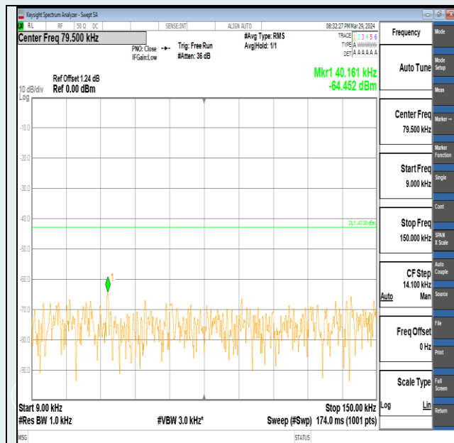
Band2-3MHz-QPSK-18615-15RB#0-0.009~0.15-PASS
