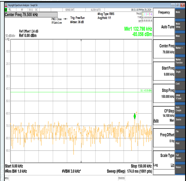
Band2-3MHz-QPSK-18615-1RB#14-0.009~0.15-PASS
