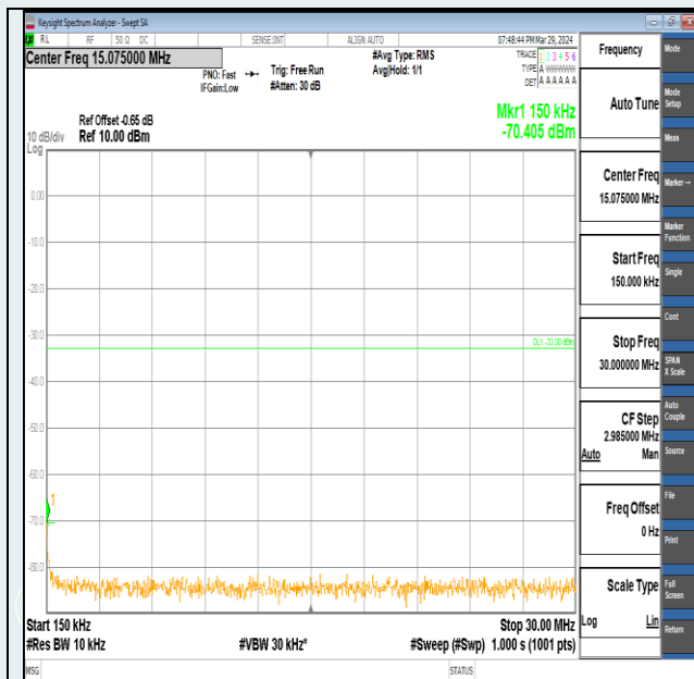
Band2-1.4MHz-16QAM-18900-1RB#5-0.15~30-PASS
