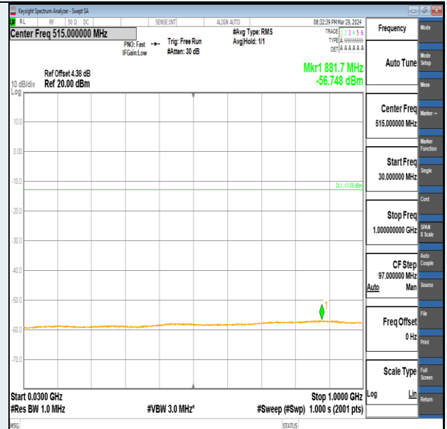
Band2-3MHz-QPSK-18615-15RB#0-30~1000-PASS
