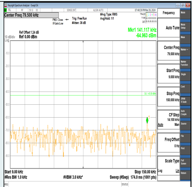
Band2-1.4MHz-16QAM-18900-1RB#5-0.009~0.15-PASS
