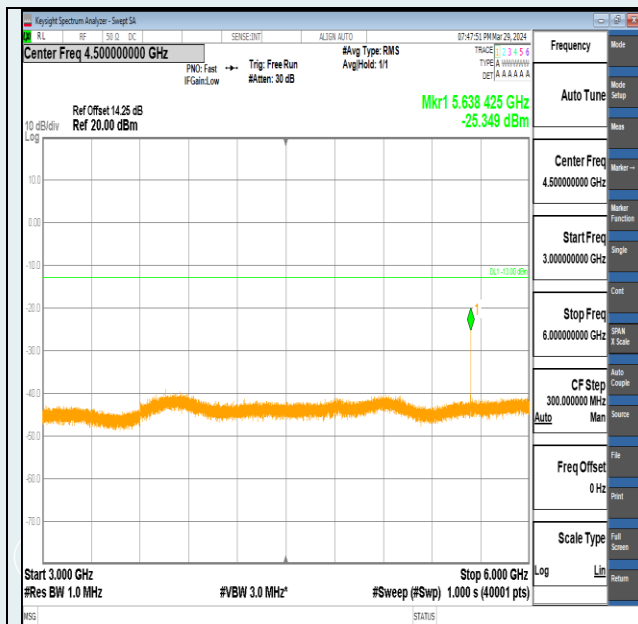
Band2-1.4MHz-16QAM-18900-1RB#0-3000~6000-PASS
