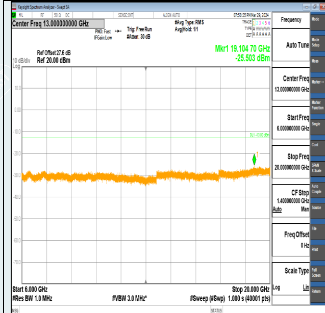
Band2-1.4MHz-QPSK-19193-6RB#0-6000~20000-PASS
