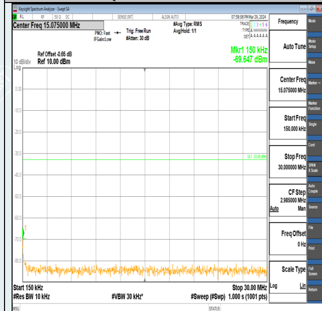
Band2-1.4MHz-QPSK-19193-6RB#0-0.15~30-PASS
