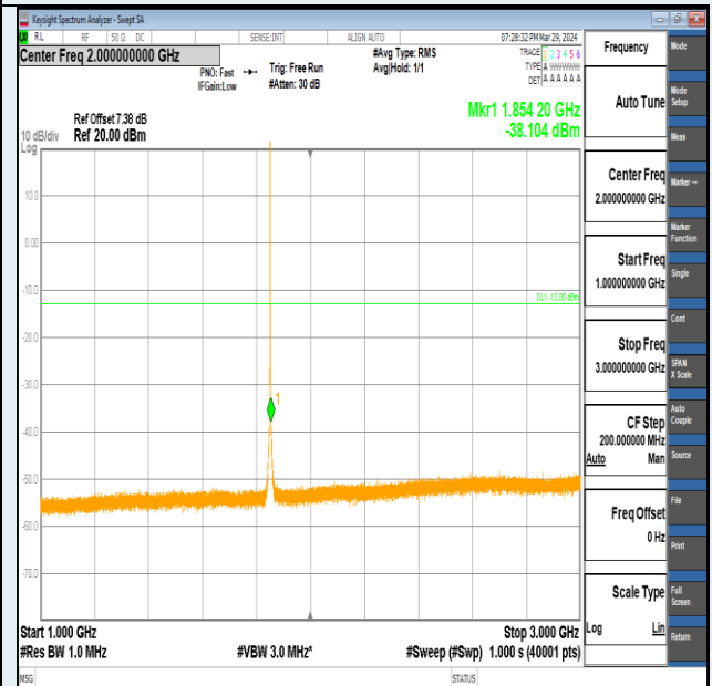
Band2-1.4MHz-QPSK-18607-1RB#5-1000~3000-PASS
