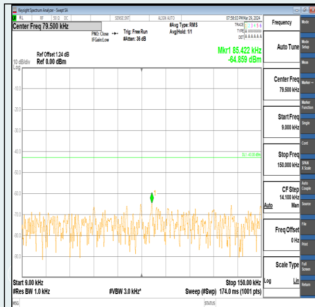
Band2-1.4MHz-QPSK-19193-6RB#0-0.009~0.15-PASS
