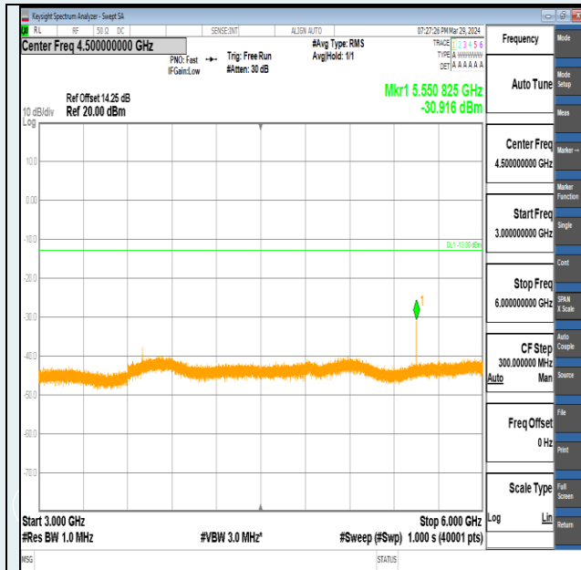
Band2-1.4MHz-QPSK-18607-1RB#0-3000~6000-PASS
