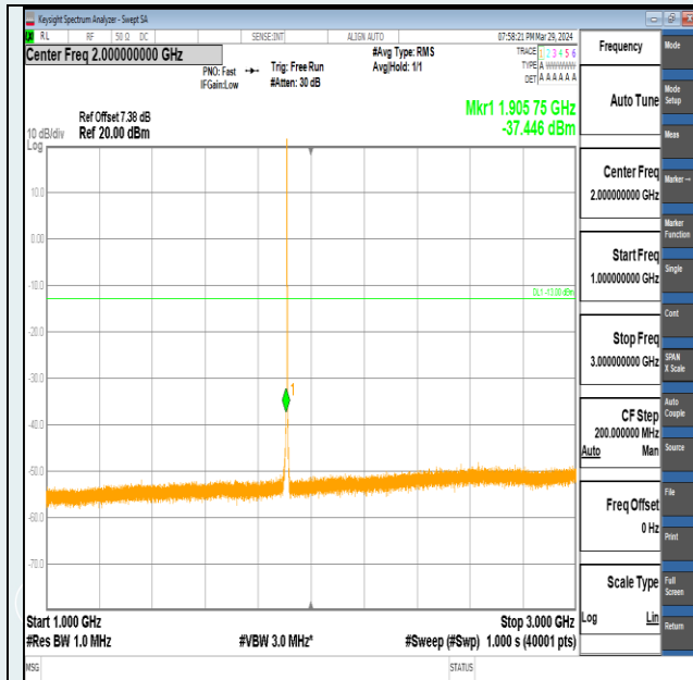
Band2-1.4MHz-QPSK-19193-6RB#0-1000~3000-PASS
