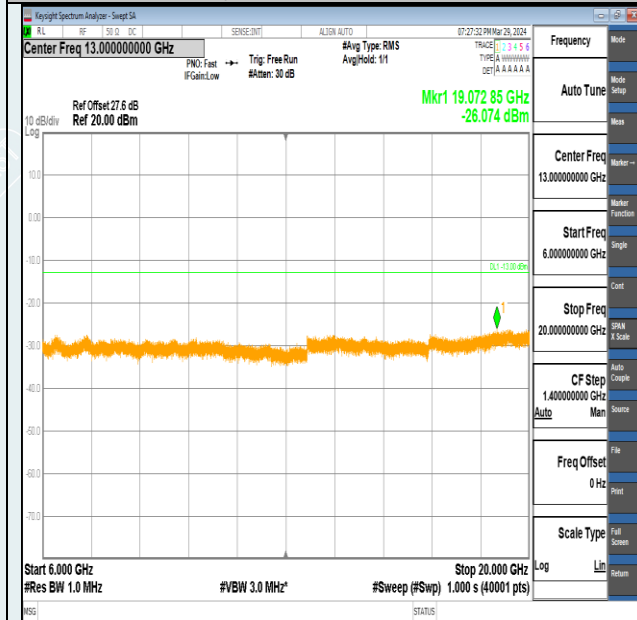
Band2-1.4MHz-QPSK-18607-1RB#0-6000~20000-PASS
