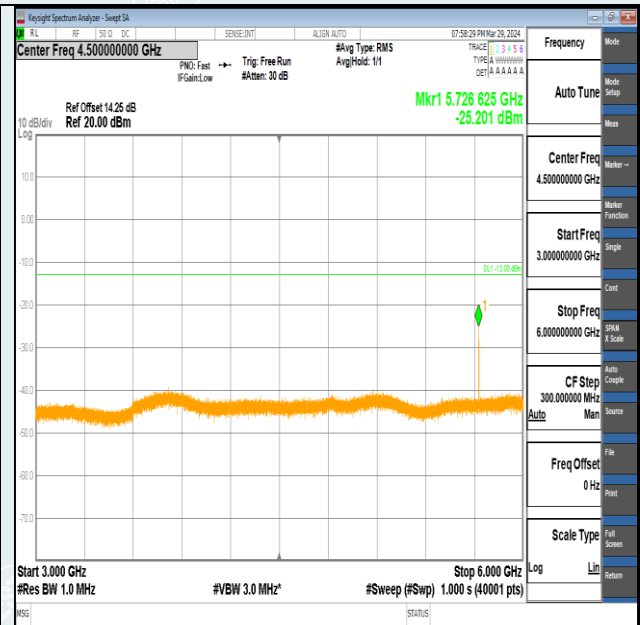
Band2-1.4MHz-QPSK-19193-6RB#0-3000~6000-PASS
