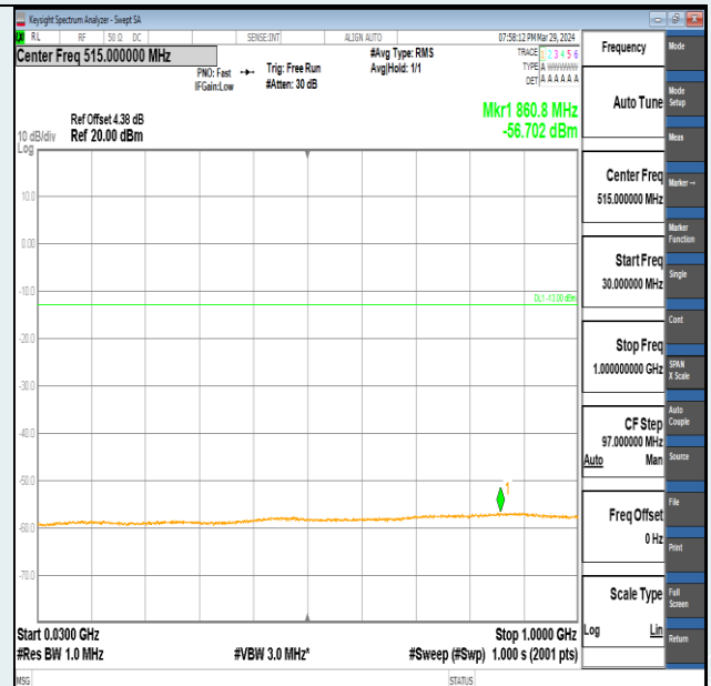
Band2-1.4MHz-QPSK-19193-6RB#0-30~1000-PASS
