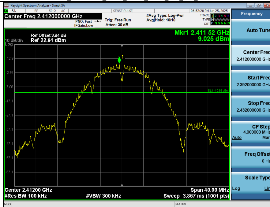
2 Bandedge_NVNT_ANT1_802_11b_2412
