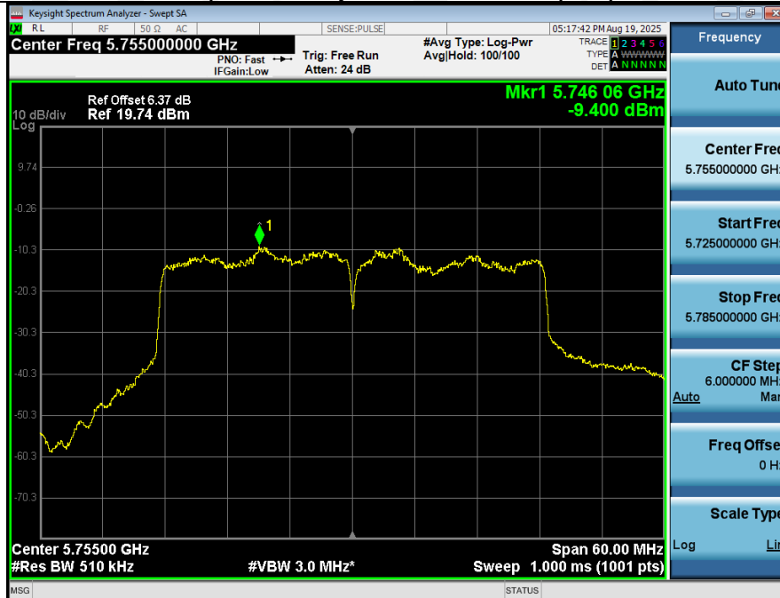
Power Spectral Density NVNT_ANT1_802_11n(HT40)_5755
