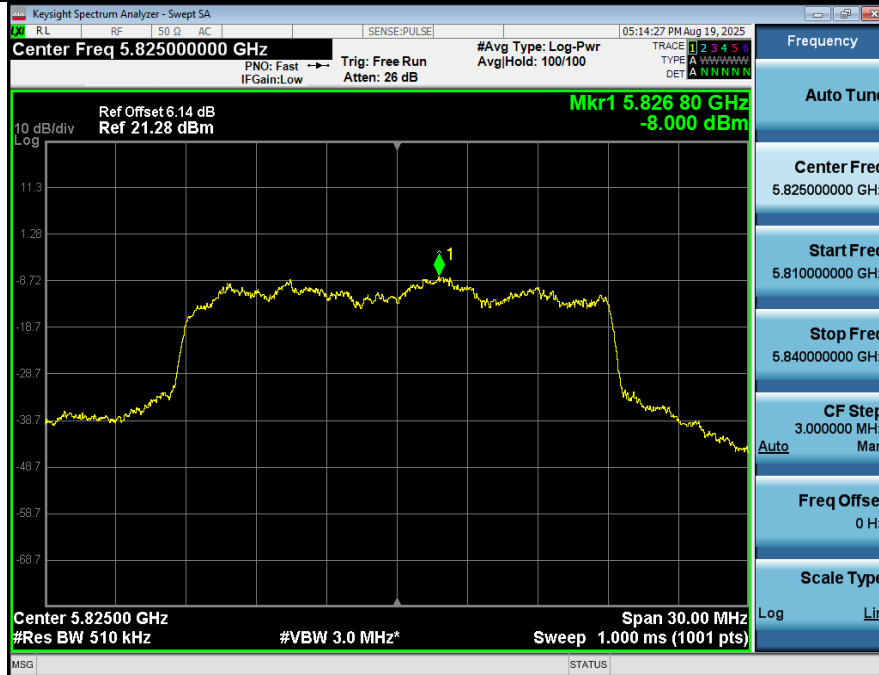
Power Spectral Density NVNT_ANT1_802_11ac(VHT20)_5825
