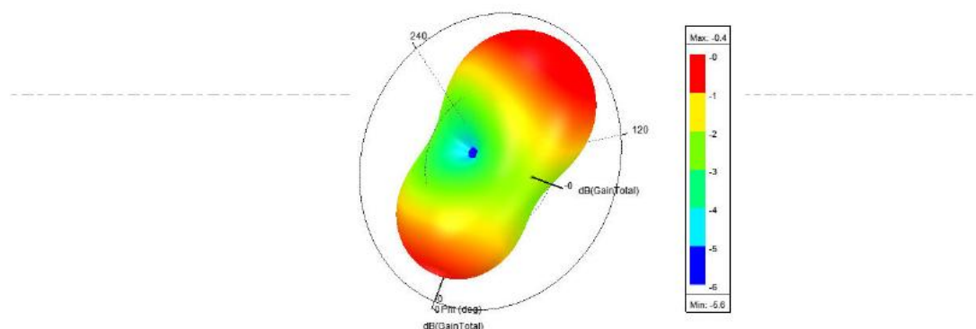
3D Gain Pattern (2450 MHz)
