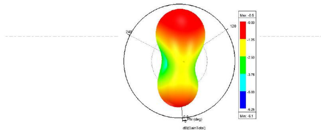
3D Gain Pattern (2500 MHz)
