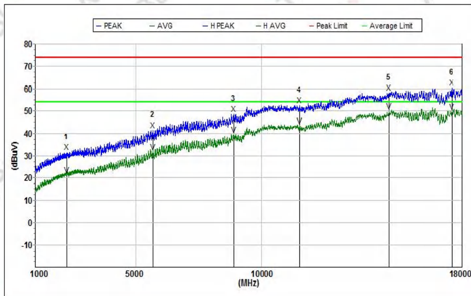
Mode 6Horizontal
