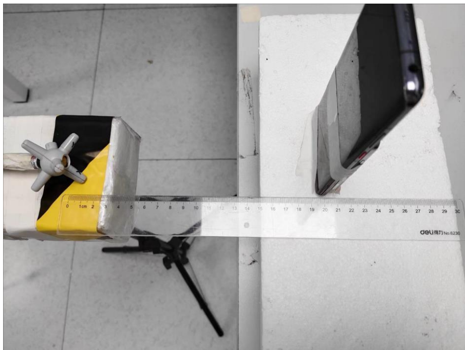
E-field Front Side (20cm)
