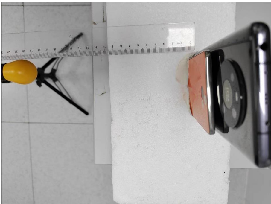
H-field Back Side (20cm)
