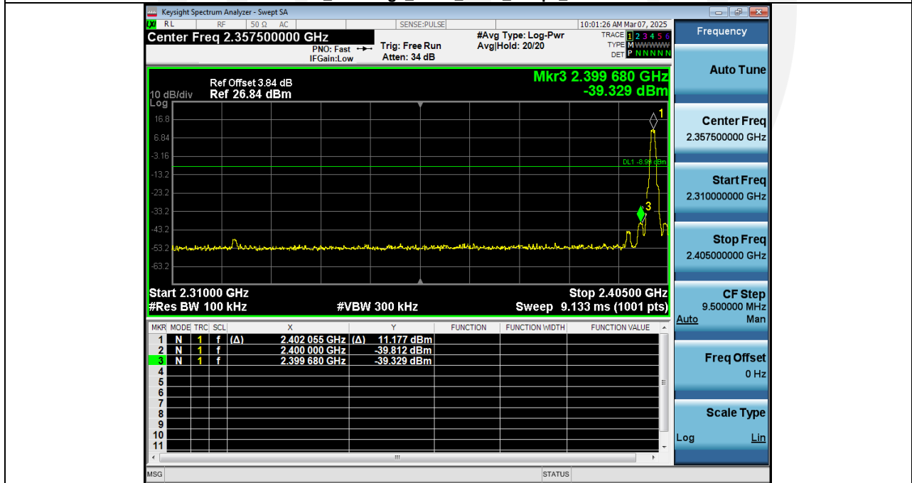
2 Bandedge_NVNT_ANT1_1Mbps_2402
