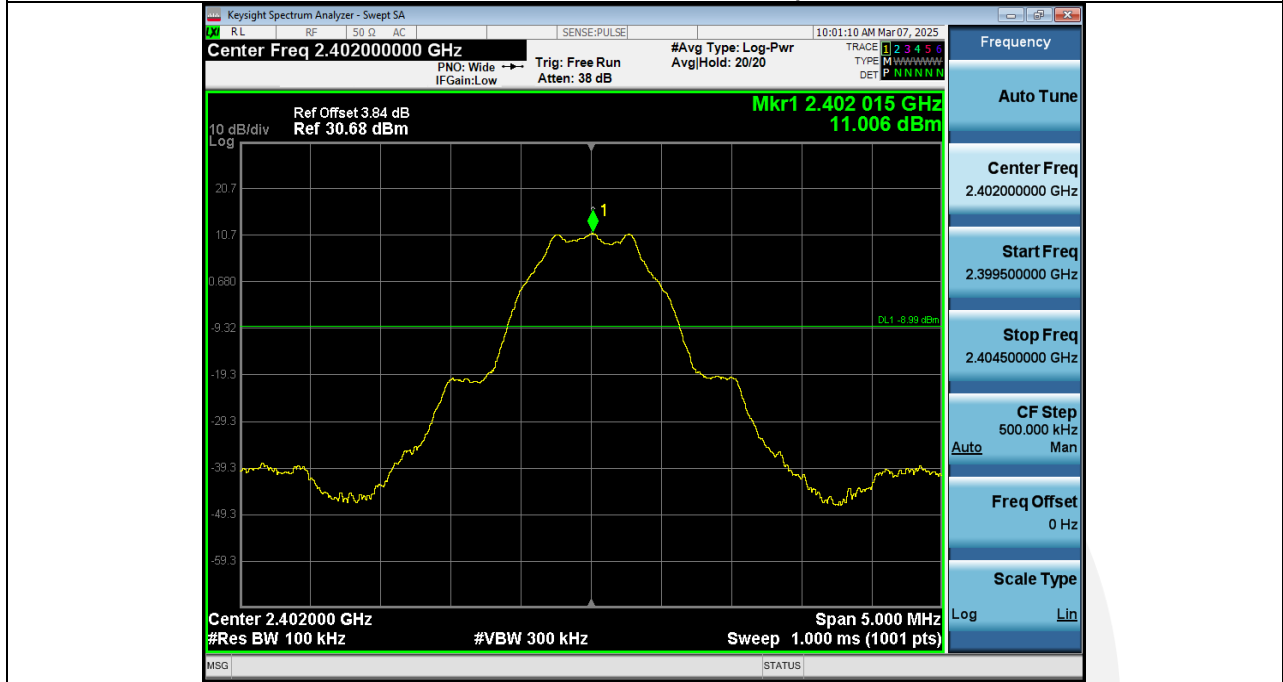
2 Bandedge_NVNT_ANT1_1Mbps_2402
