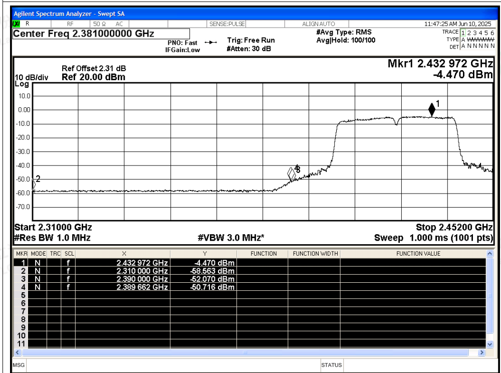
Restrict Band NVNT ax40 2422MHz Ant2 Average
