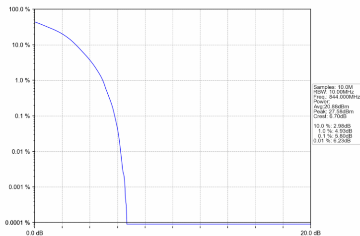
Band5 10MHz 16QAM HCH 844MHz RB 27 23 NTNV
