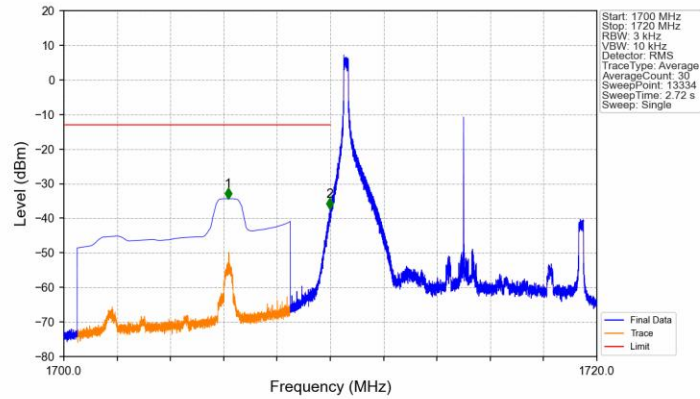
Band4 10MHz QPSK LCH 1715MHz RB 1 0 NTN
