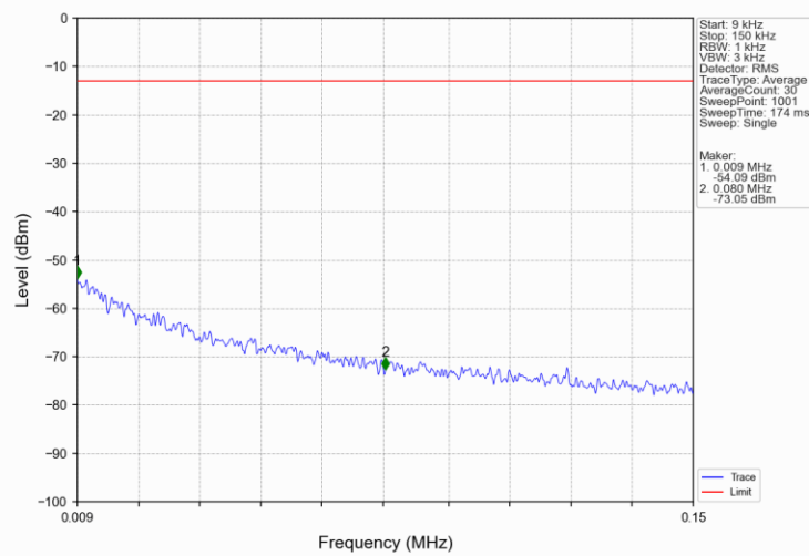
Band4_5MHz_QPSK_LCH_1712.5MHz_RB_1_0 NTN
